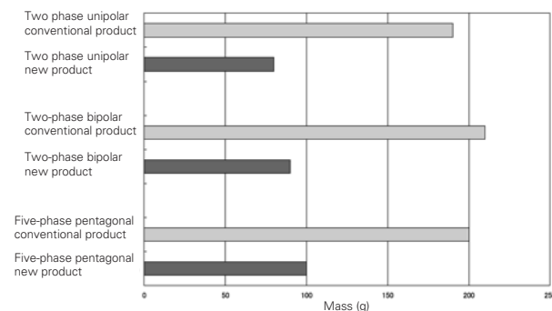
Figure 4 Weight comparison
