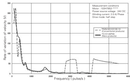
Figure 7 Vibration characteristics
