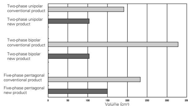
Figure 3 Size comparison
