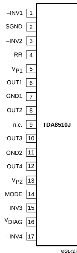
Fig.2 Pin configuration.
