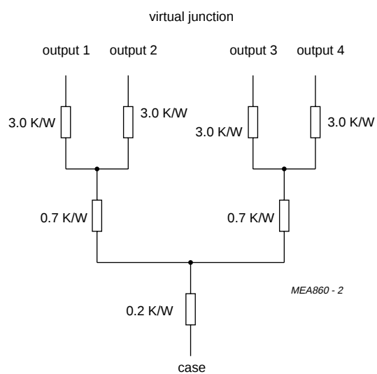
Fig.6 Equivalent thermal resistance network.
