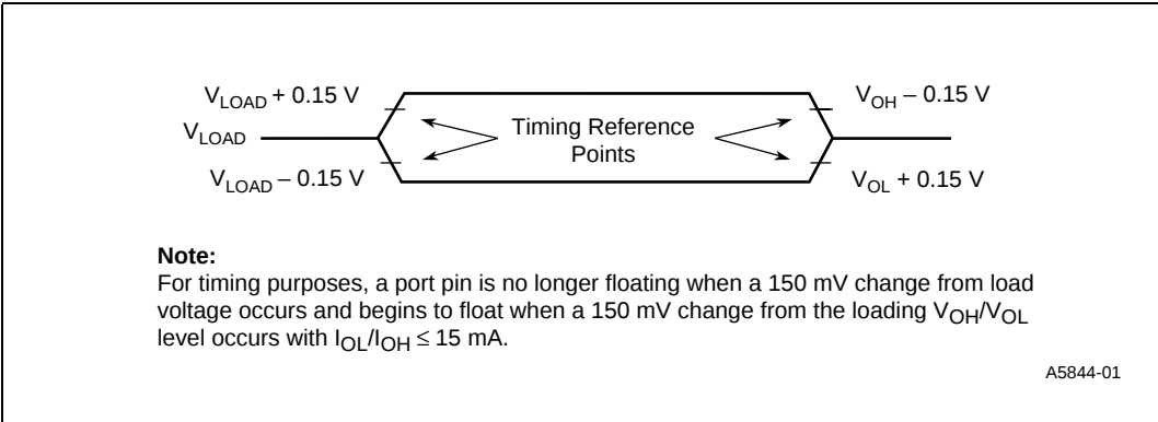
Figure 13. Float Waveforms
