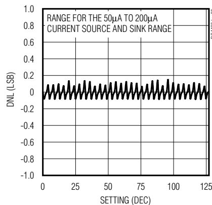
DIFFERENTIAL LINEARITY
