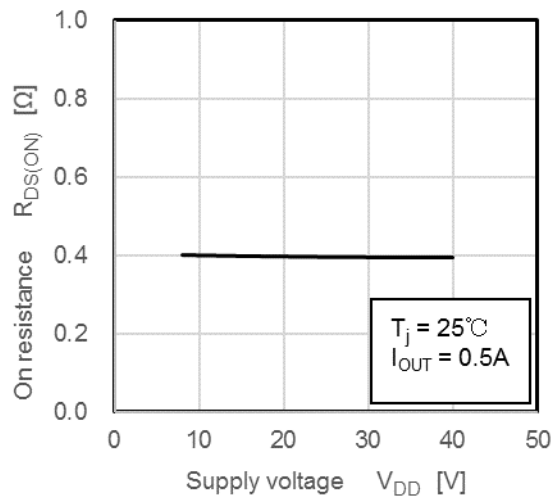
R_{DS(ON)} - V_{DD}
