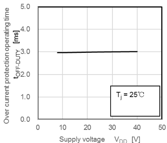
t_{OFF-DUTY} - V_{DD}
