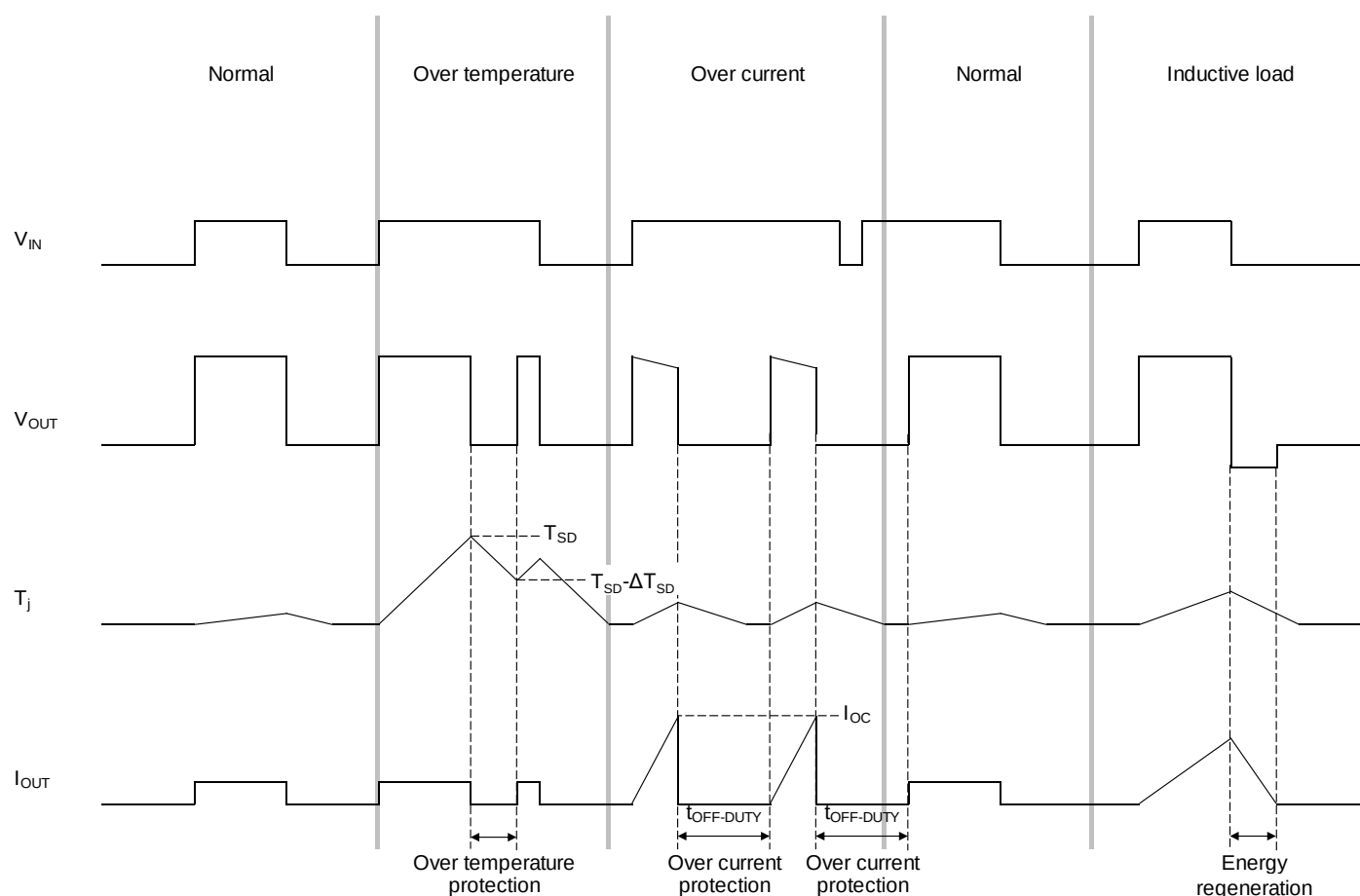
Figure 7.1 Timing chart
