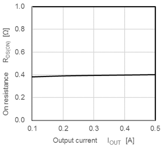
R_{DS(ON)} - I_{OUT}
