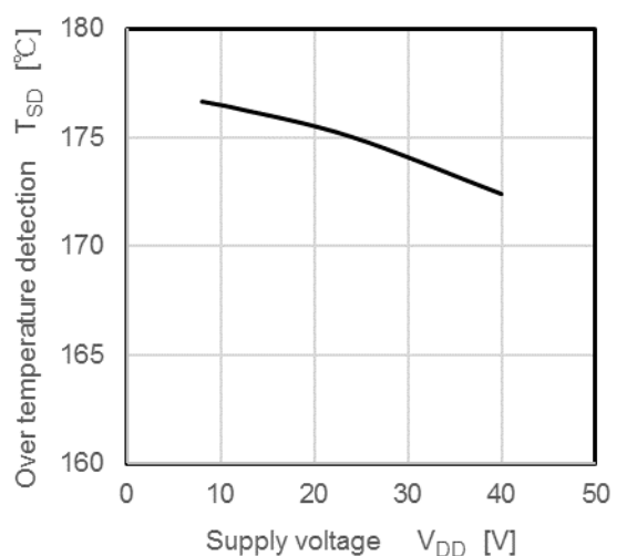
T_{SD} - V_{DD}
