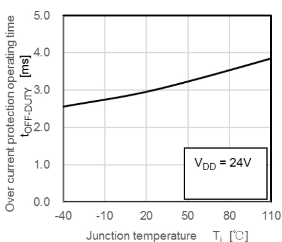
t_{OFF-DUTY} - T_j
