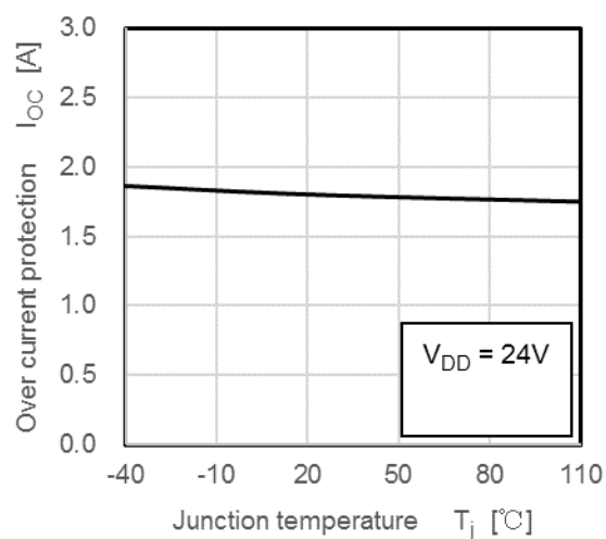
I_{OC} - T_j
