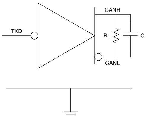
Figure 7-3. Supply Test Circuit
