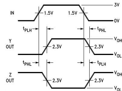
Figure 7. Driver Propagation Times( 2 )( 4 )
