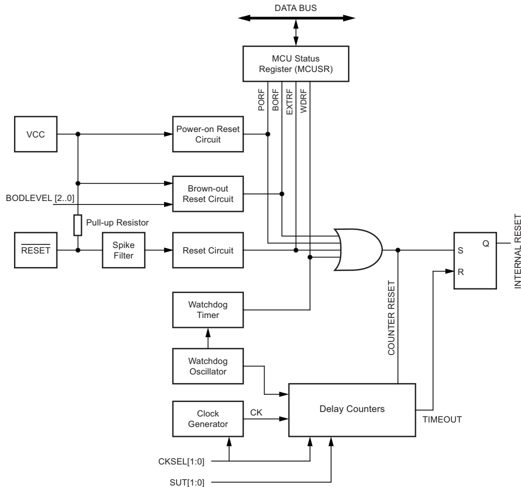
Figure 8-1. Reset Logic
