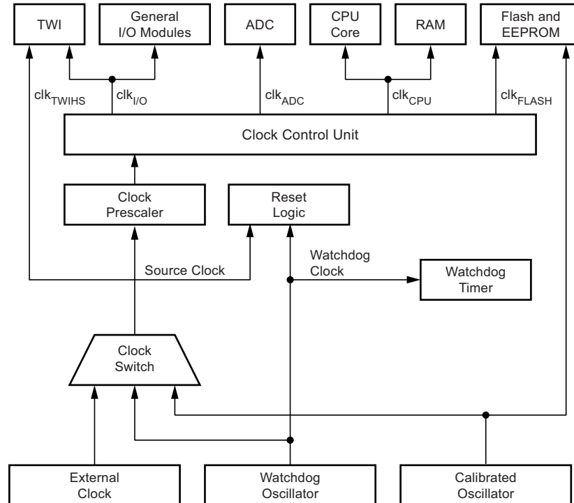
Figure 6-1. Clock Distribution
