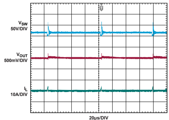
Figure 9. Burst Mode Waveforms
