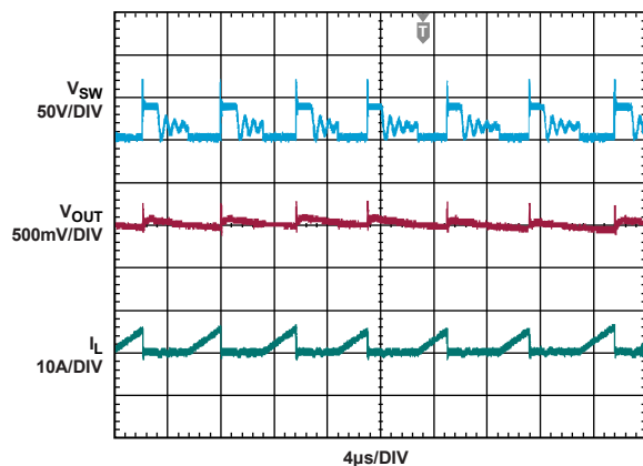
Figure 8. Discontinuous Mode Waveforms
