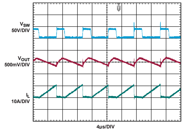
Figure 7. Boundary Mode Waveforms
