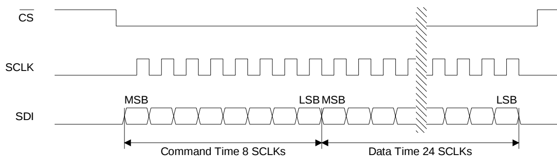
Write Cycle
