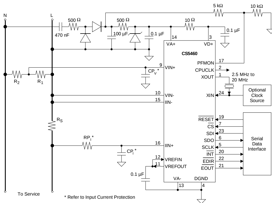
Figure 3. Typical Connection Diagram (One-Phase 2-Wire)
