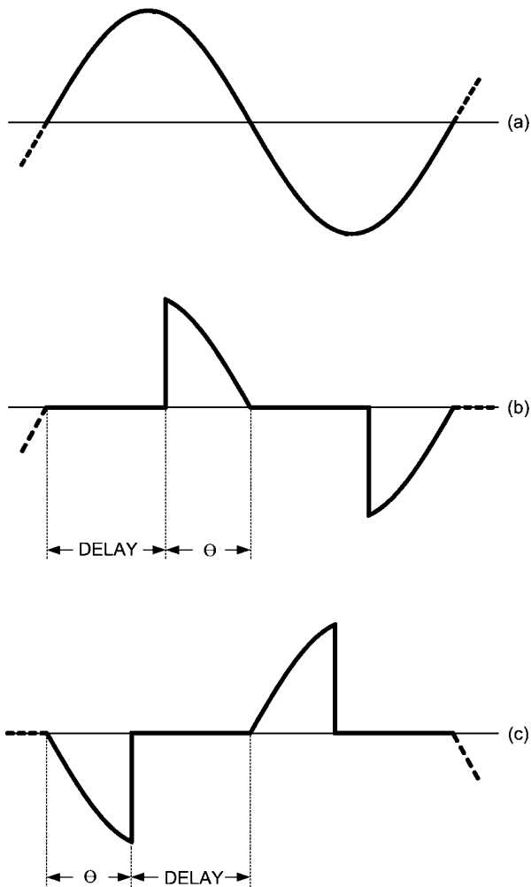
FIGURE 3. Line Voltage and Dimming Waveforms
