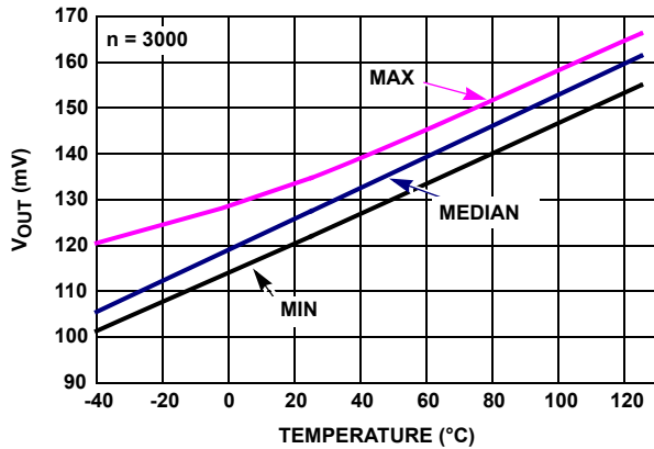
FIGURE 33. ISL28271 V_{OUT} LOW vs TEMPERATURE, R_L = 1k , V_+ = \pm 2.5V
