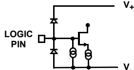
CIRCUIT 2
