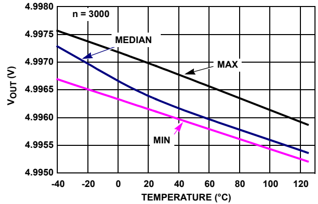
FIGURE 32. ISL28272 V_{OUT} HIGH vs TEMPERATURE, R_L = 100k , V_+ = \pm 2.5V
