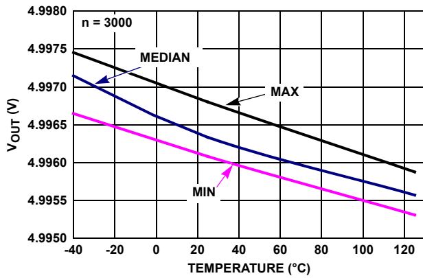
FIGURE 31. ISL28271 V_{OUT} HIGH vs TEMPERATURE, R_L = 100k , V_+ = \pm 2.5V
