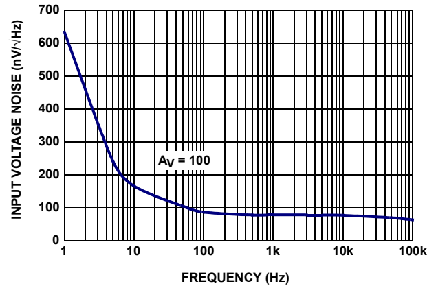
FIGURE 16. ISL28272 INPUT VOLTAGE NOISE SPECTRAL DENSITY
