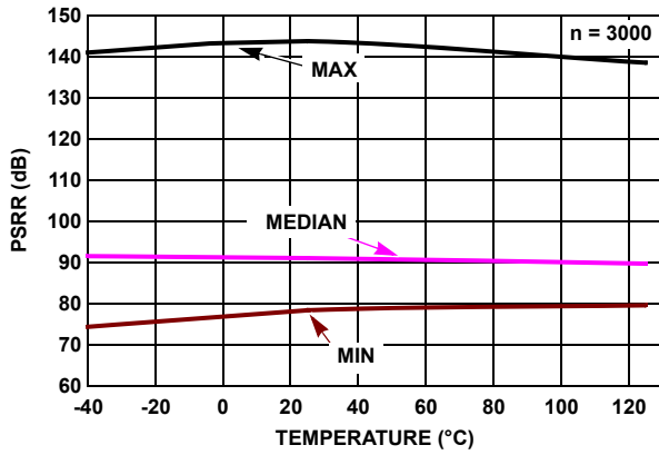
FIGURE 27. ISL28271 PSRR vs TEMPERATURE, V_+, V_- = \pm 1.2V TO \pm 2.5V
