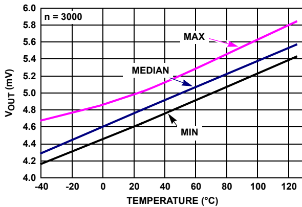
FIGURE 35. ISL28271 V_{OUT} LOW vs TEMPERATURE, R_L = 100k , V_+ = \pm 2.5V
