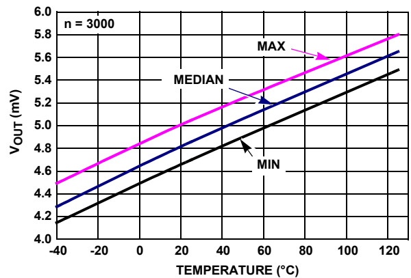
FIGURE 36. ISL28272 V_{OUT} LOW vs TEMPERATURE, R_L = 100k , V_+ = \pm 2.5V
