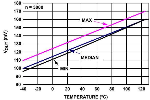
FIGURE 34. ISL28272 V_{OUT} LOW vs TEMPERATURE, R_L = 1k , V_+ = \pm 2.5V
