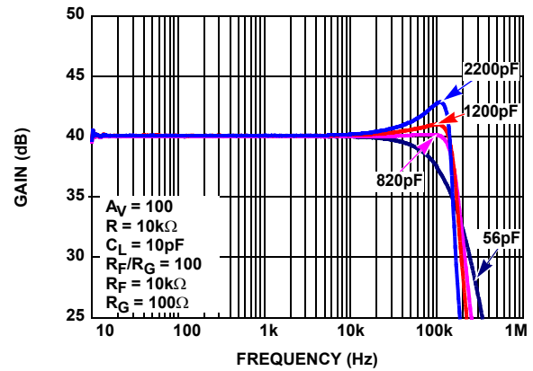
FIGURE 10. ISL28272 FREQUENCY RESPONSE vs C_{LOAD}
