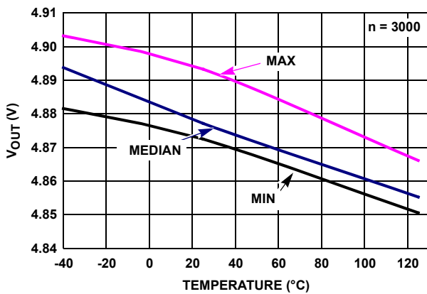
FIGURE 29. ISL28271 V_{OUT} HIGH vs TEMPERATURE, R_L = 1k , V_+, V_- = \pm 2.5V
