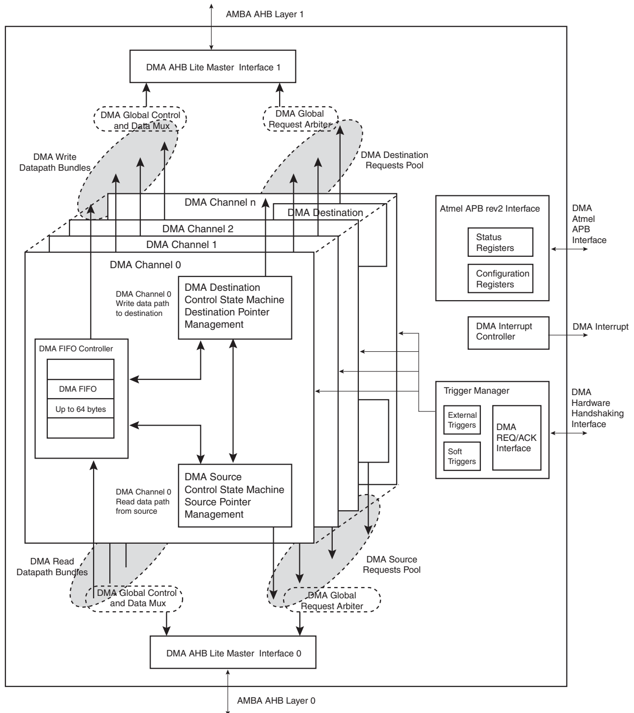
Figure 41-1. DMA Controller (DMAC) Block Diagram
