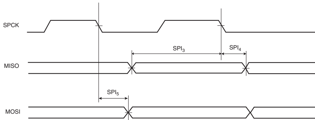
Figure 46-7. SPI Slave Mode 0 and 3)
