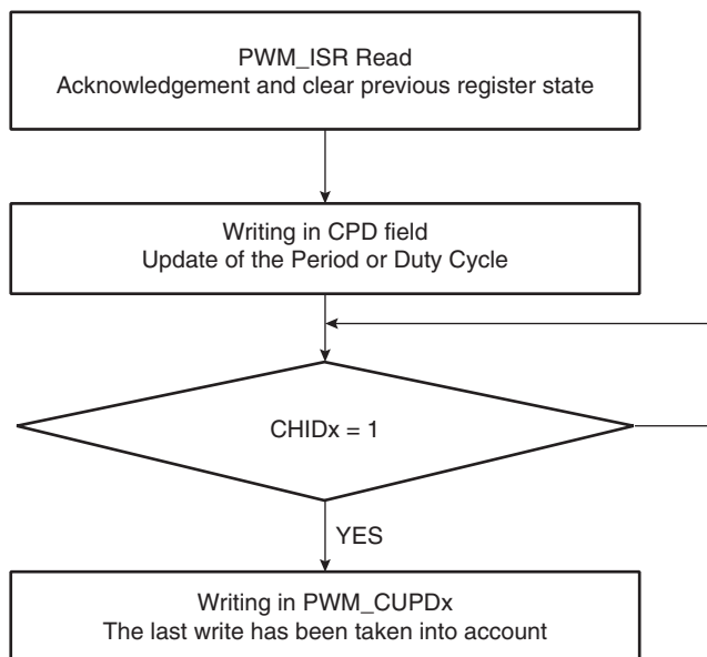
Figure 42-7. Polling Method
