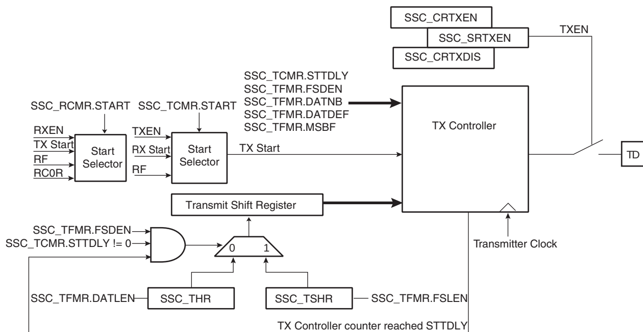
Figure 34-9. Transmitter Block Diagram
