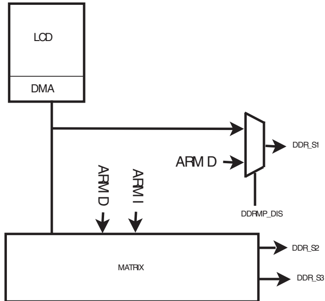
Figure 19-1. DDR Multi-port
