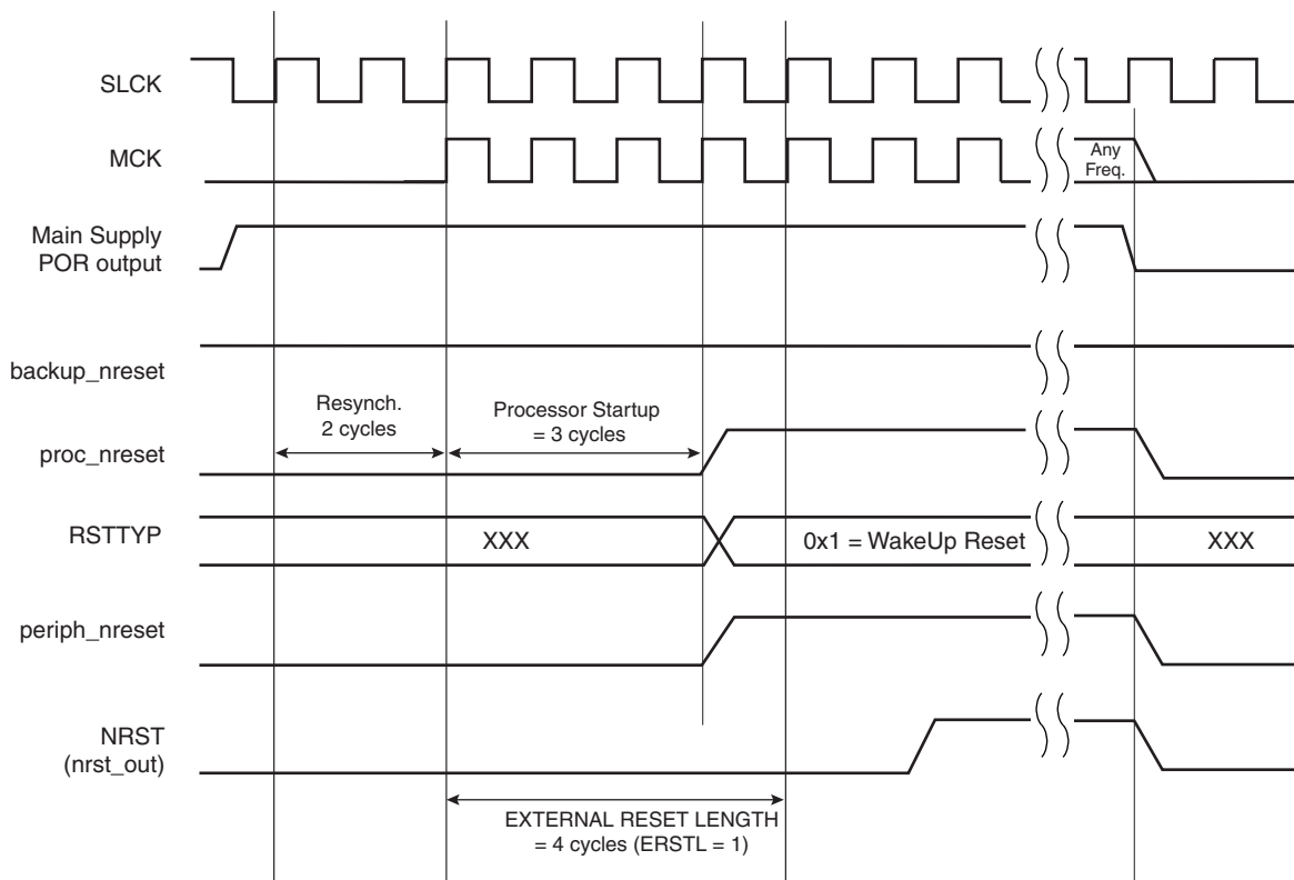
Figure 12-5. Wake-up State
