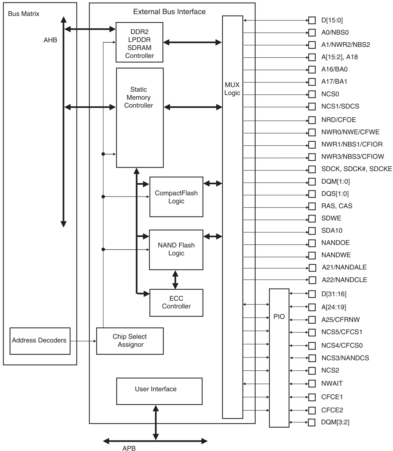
Figure 20-2. Organization of the External Bus Interface
