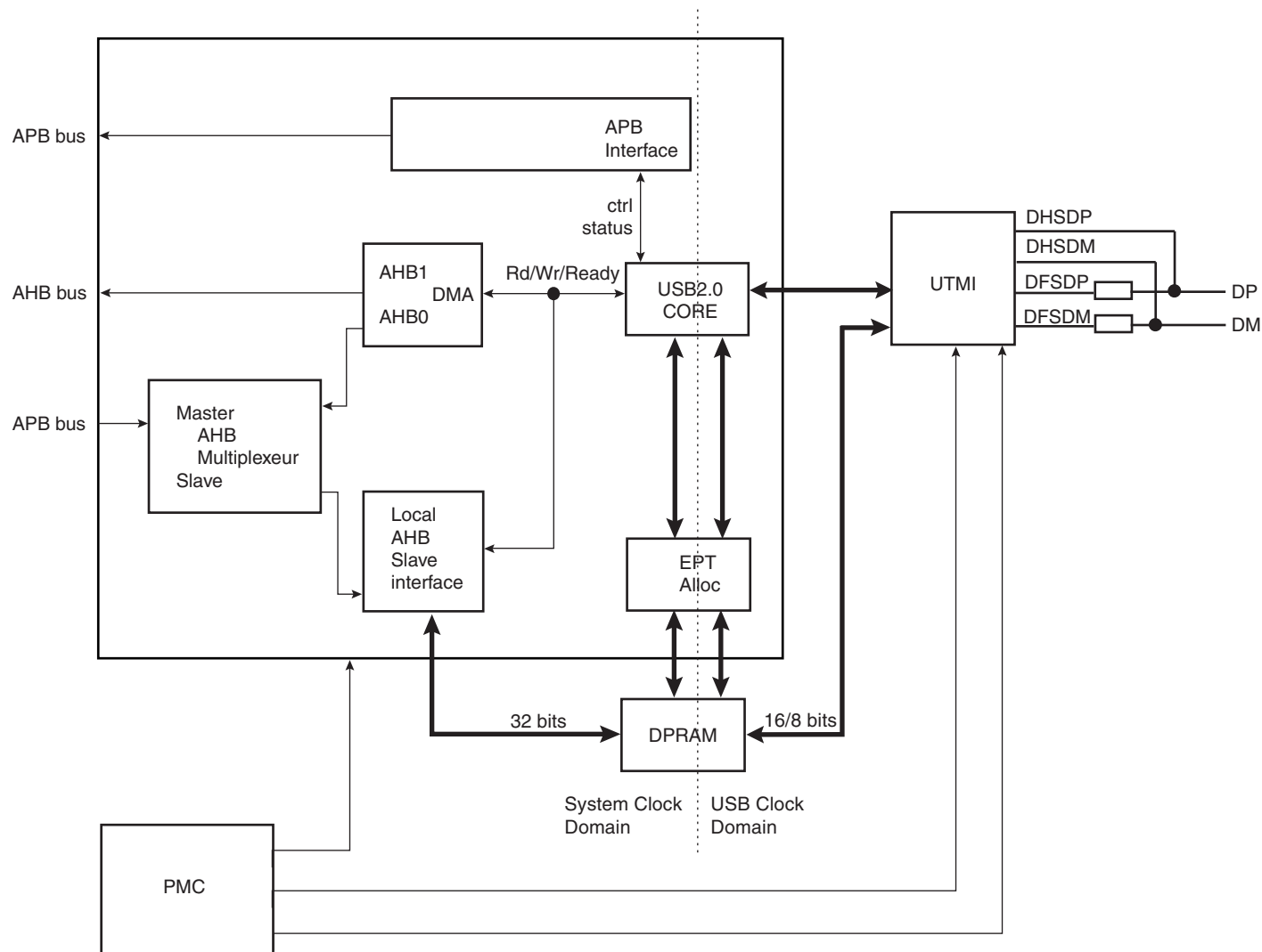
Figure 38-2. Block Diagram
