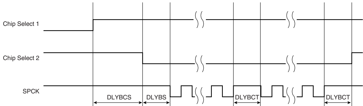
Figure 30-10. Programmable Delays
