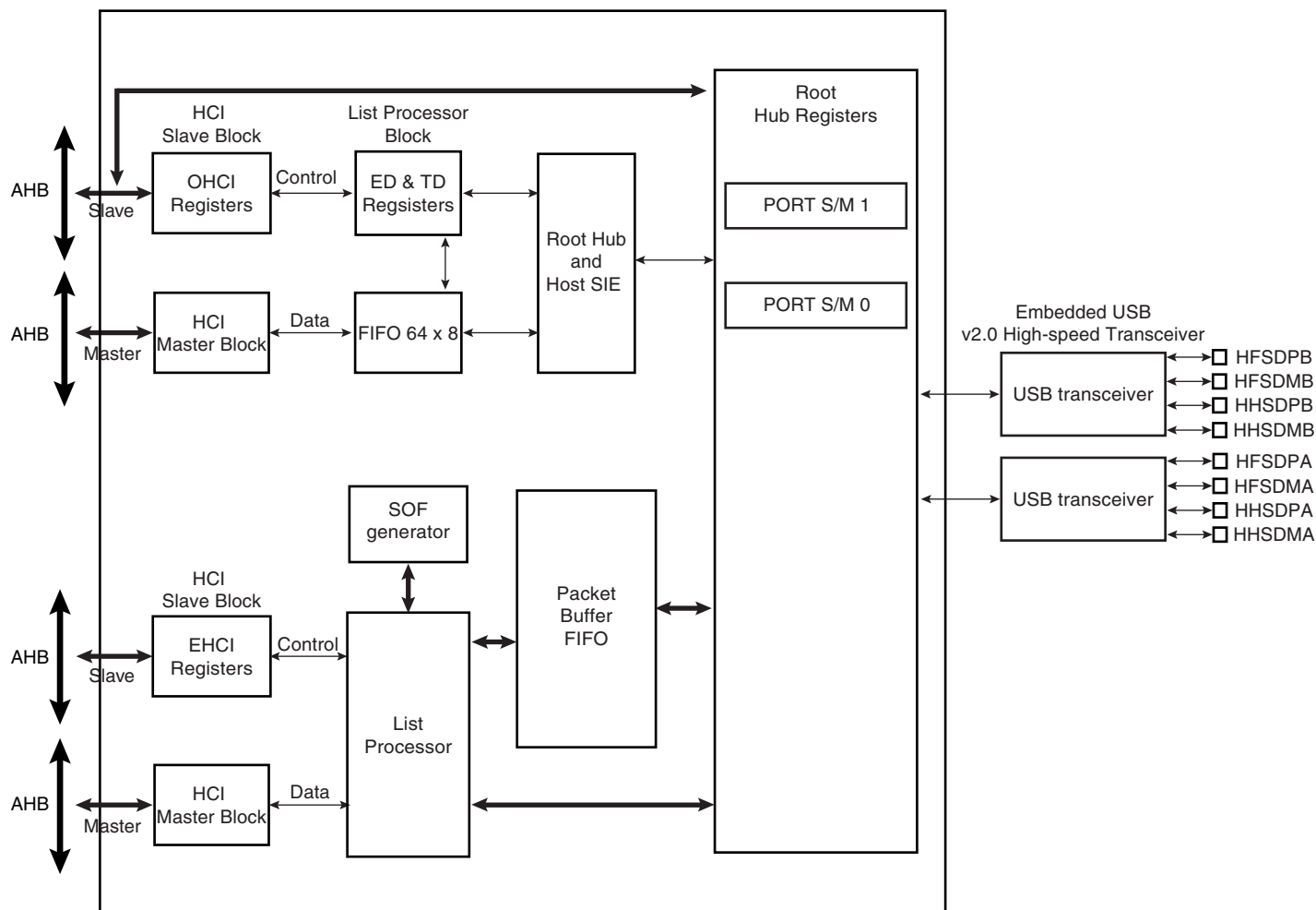
Figure 37-2. Block Diagram
