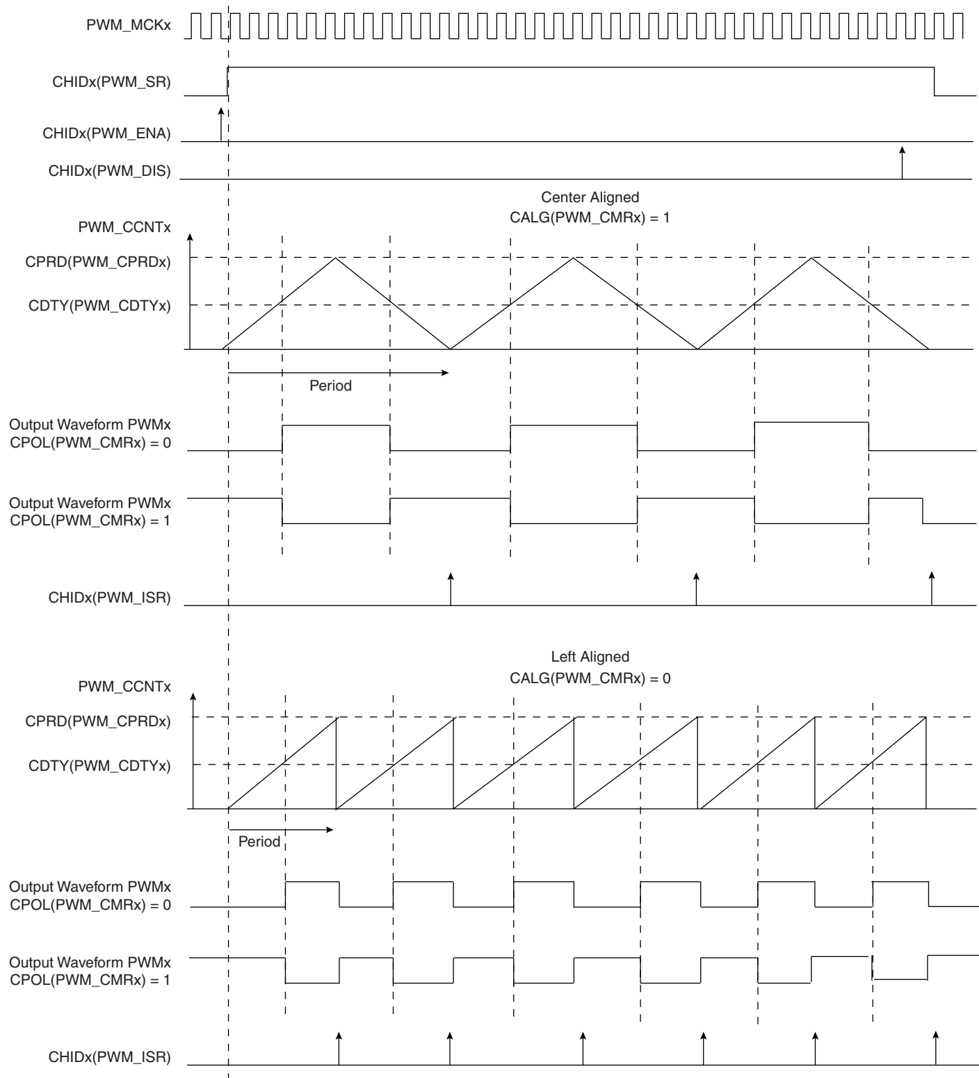
Figure 42-5. Waveform Properties
