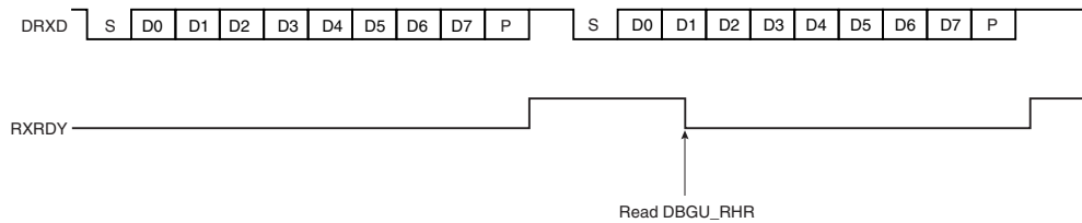
Figure 28-6. Receiver Ready
