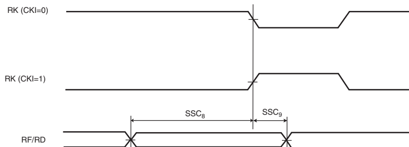
Figure 46-14. SSC Receiver RK and RF in Input
