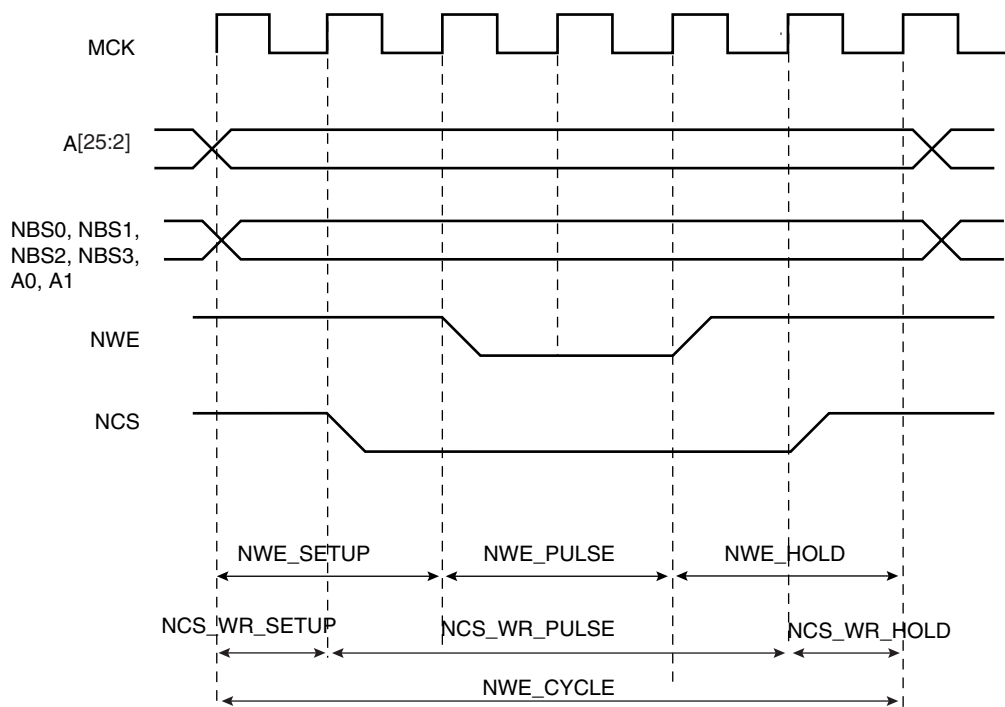
Figure 21-12. Write Cycle
