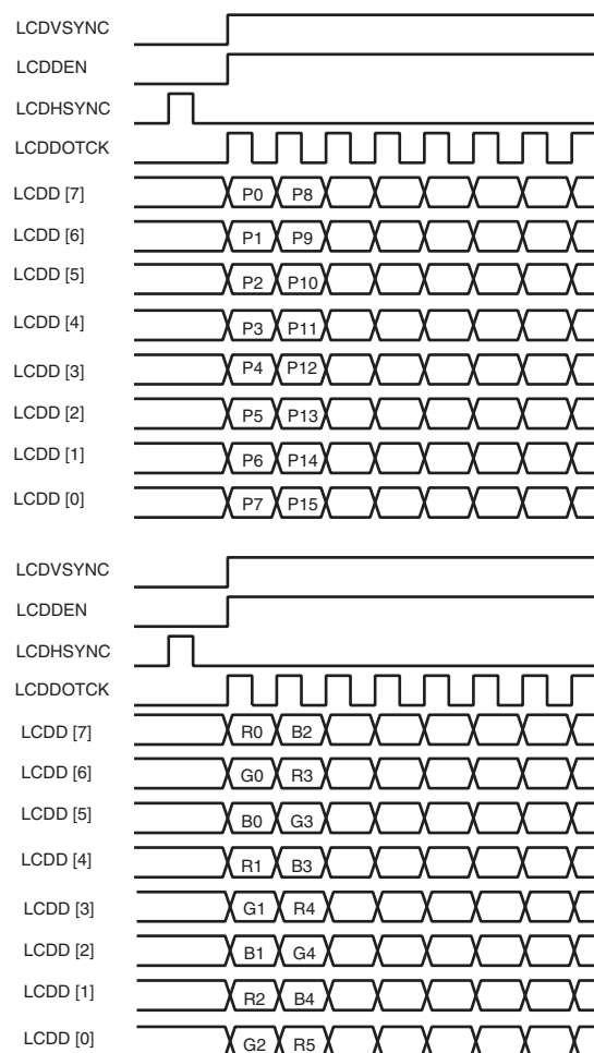
Figure 45-10. Single Scan Monochrome and Color 8-bit Panel Timing (First Line Expanded View)
