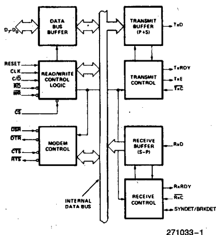
Figure 1. Block Diagram
