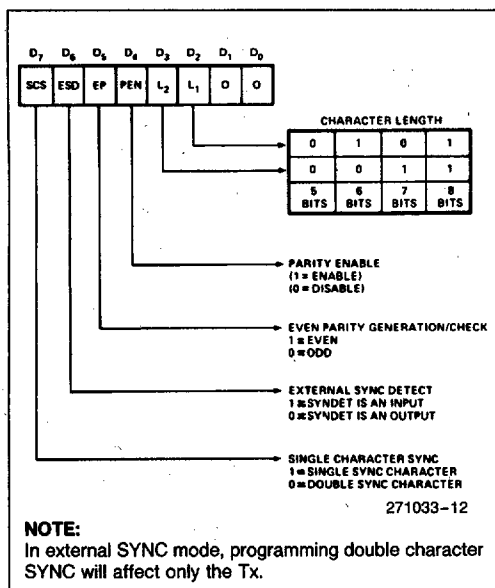
Figure 10. Mode Instruction Format, Synchronous Mode
