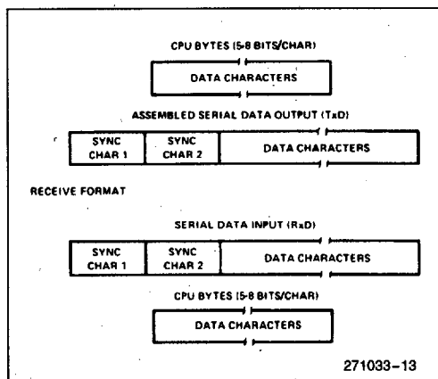
Figure 11. Data Format, Synchronous Mode
