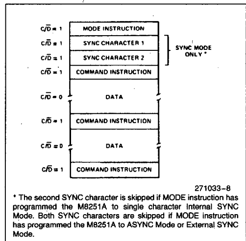
Figure 7. Typical Data Block
