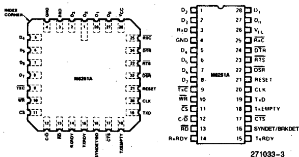
Figure 2. Pin Configurations
