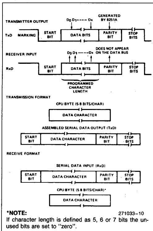
Figure 9. Asynchronous Mode
