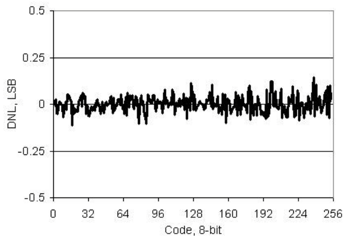
Figure 11-35. IDAC DNL vs Input Code, Range = 255 \mu A, Sink Mode
