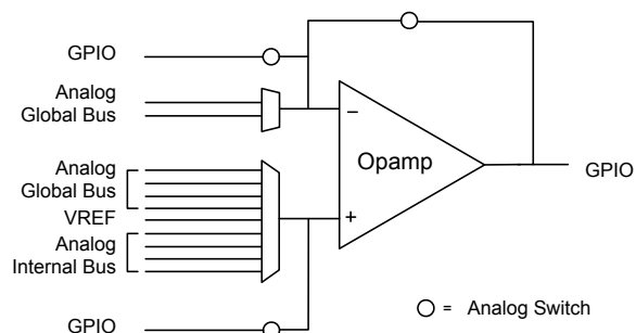
Figure 8-7. Opamp
