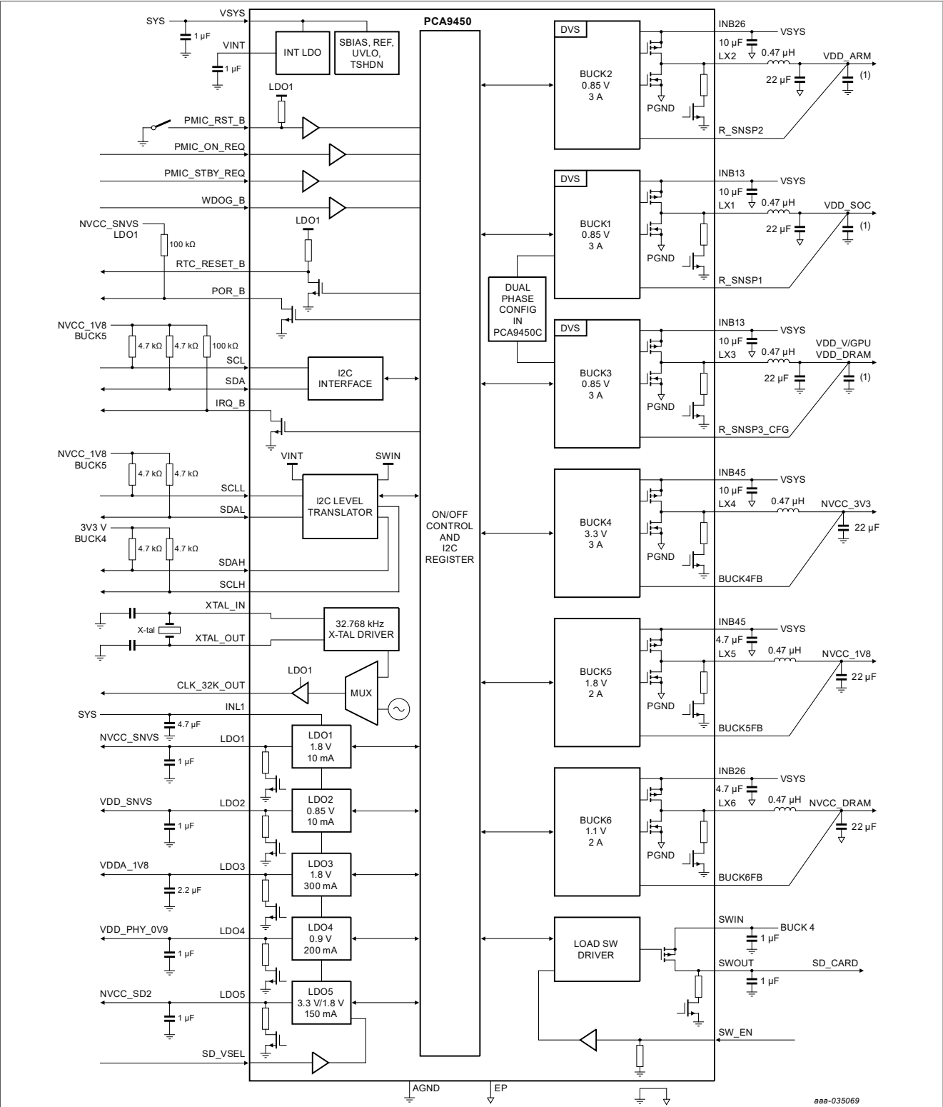
Figure 1. Block diagram
