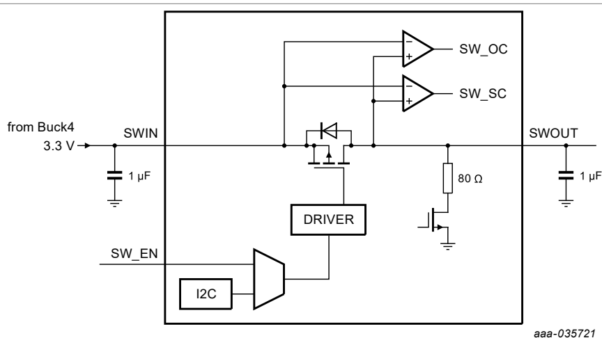
Figure 18. Load switch internal block diagram
