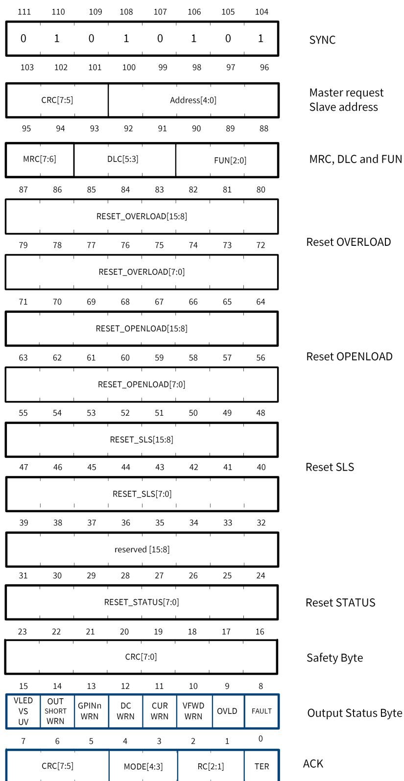
Figure 25 Hardware control frame
