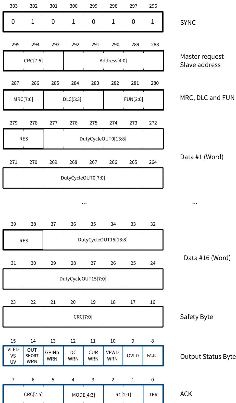
Figure 23 Update duty cycle (DC_UPDATE) for DLC = 0x06
