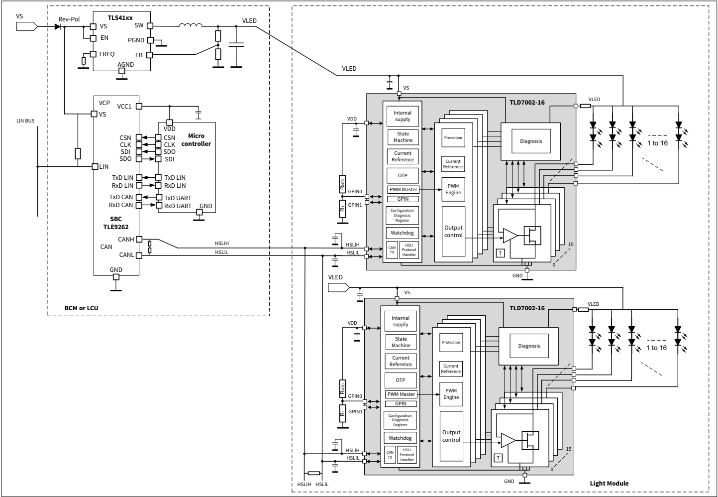
Figure 40 Application diagram
