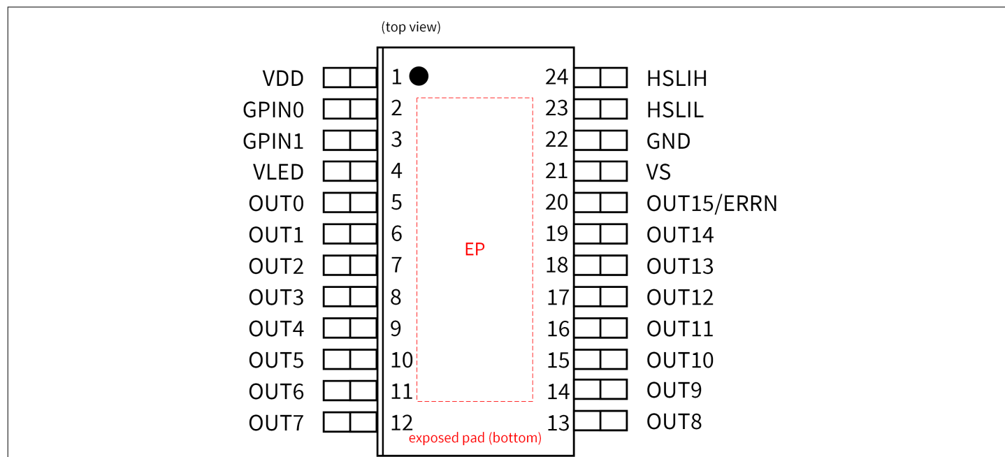
Figure 3 Pin configuration
