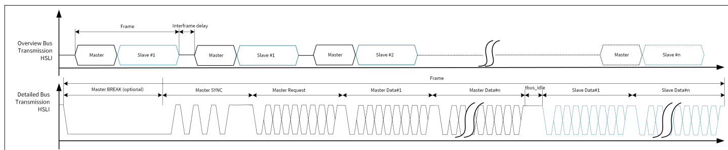
Figure 17 Structure of a frame
