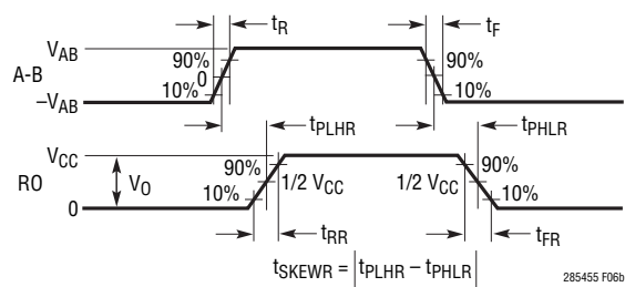
Figure 6. Receiver Propagation Delay Measurements
