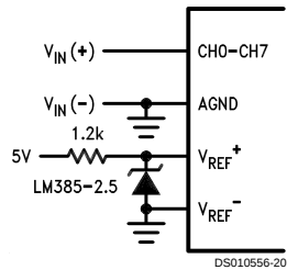
External Reference 2.5V Full Scale
