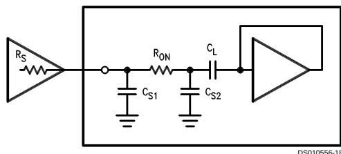
FIGURE 1. Analog Input Model
