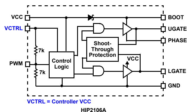
Figure 1. Block Diagrams
