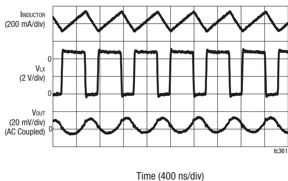
Figure 23. Buck 1 Output Ripple ( V_{IN} = 5.0\text{ V} , V_{OUT} = 3.0\text{ V} , C_{OUT} = 4.7\text{ }\mu\text{F} , 400 mA Load)
