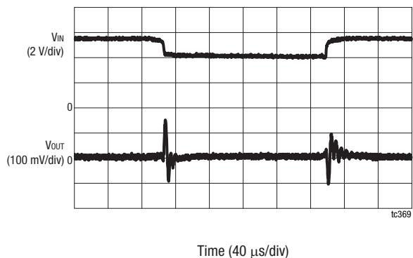
Figure 31. Buck 3 Line Transient Response ( V_{IN} = 4.1\text{ V to } 5.0\text{ V} , V_{OUT} = 1.2\text{ V} , 300 mA Load)
