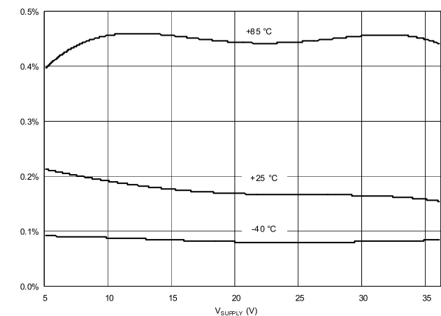
Figure 9. Output Error vs. Supply Voltage
