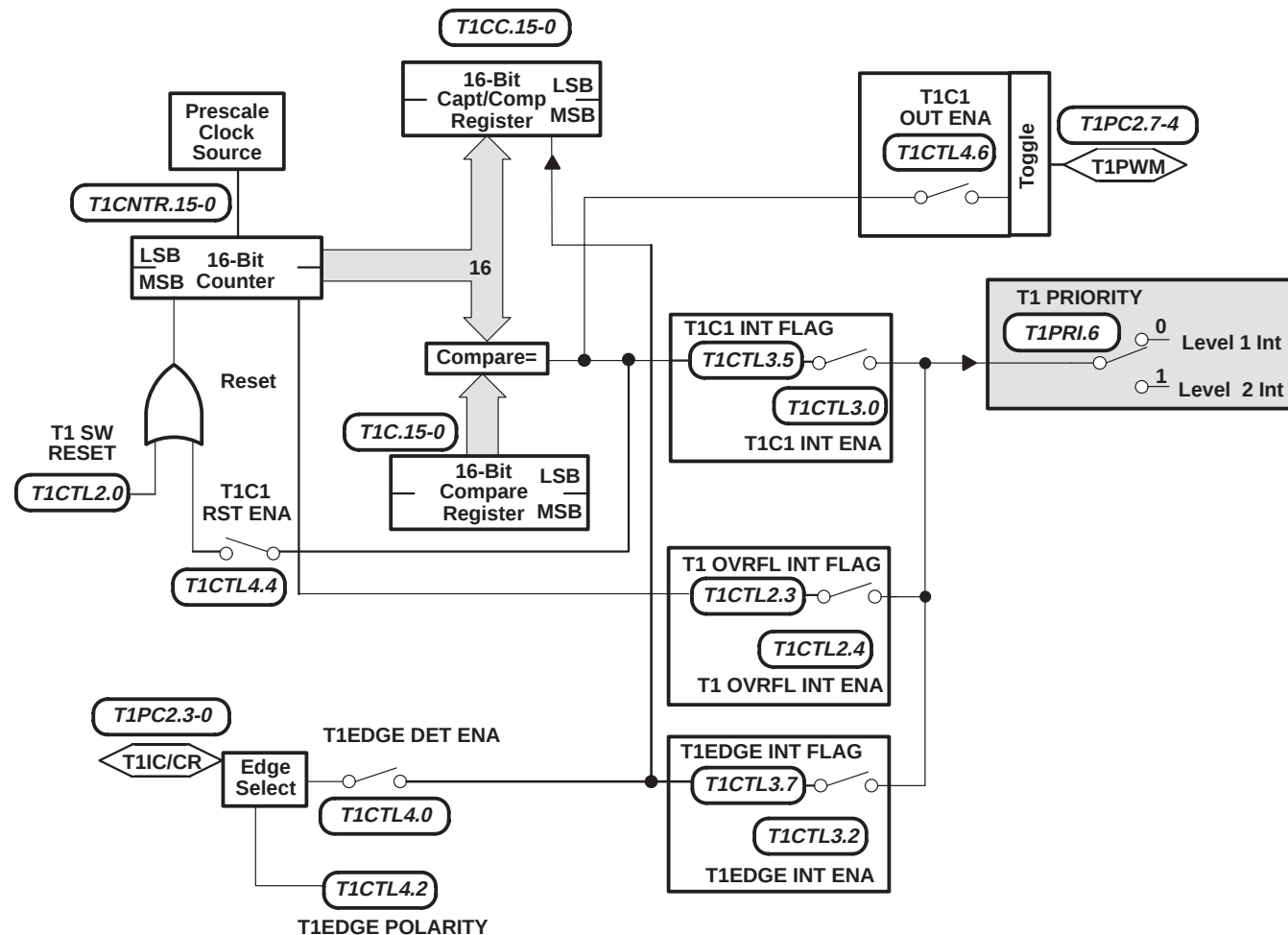
Figure 6. Capture/Compare Mode
