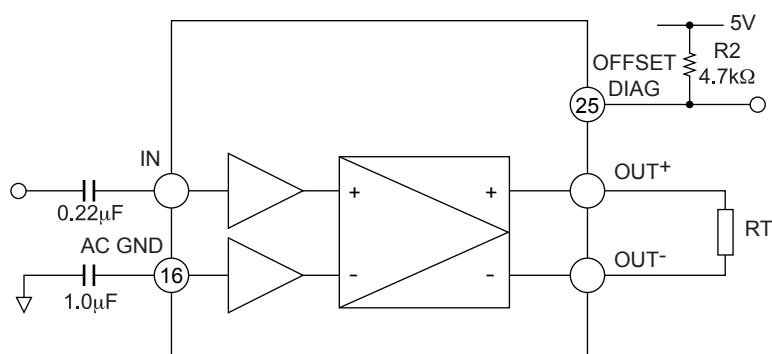
Fig4 Operating Pin 25
