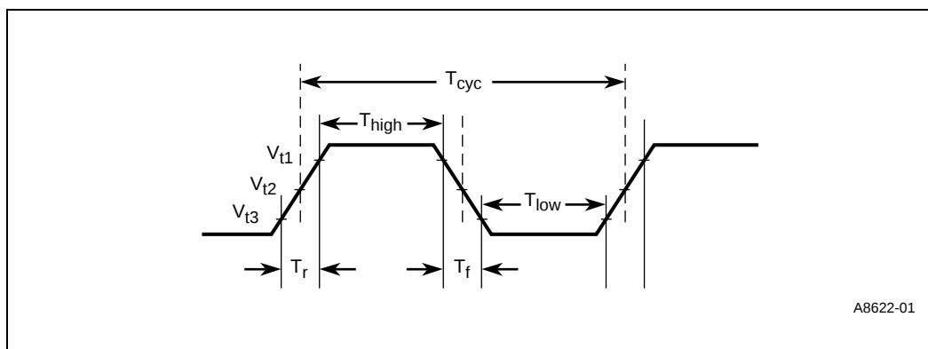
Figure 75. SDCLK AC Timing Diagram
