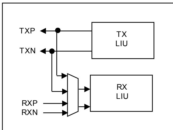
Figure 10-10. ALB Mux
