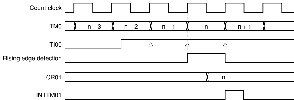
Figure 6-17. Capture Operation of CR01 with Rising Edge Specified
