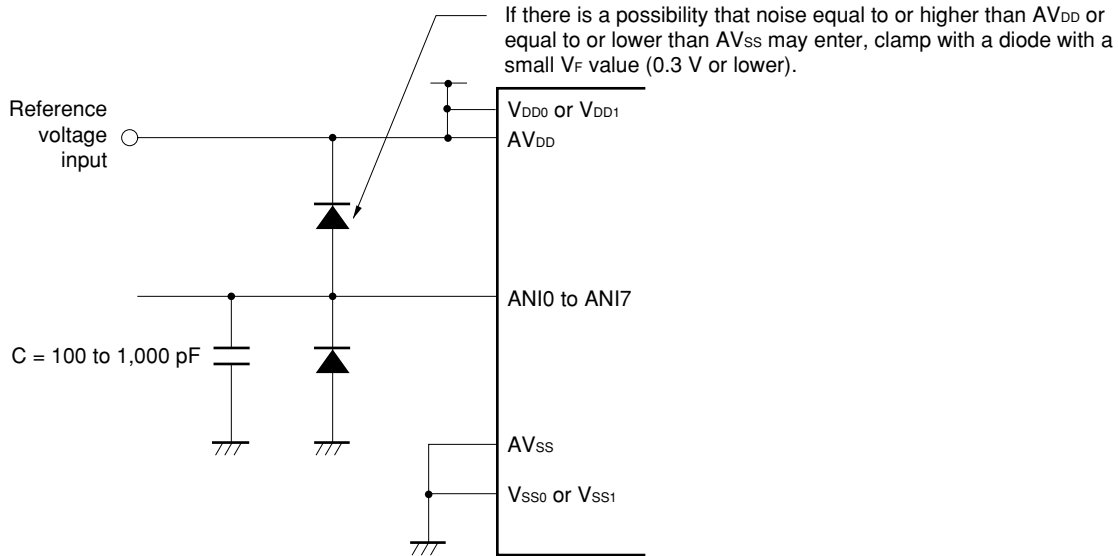
★ Figure 13-16. Analog Input Pin Connection
