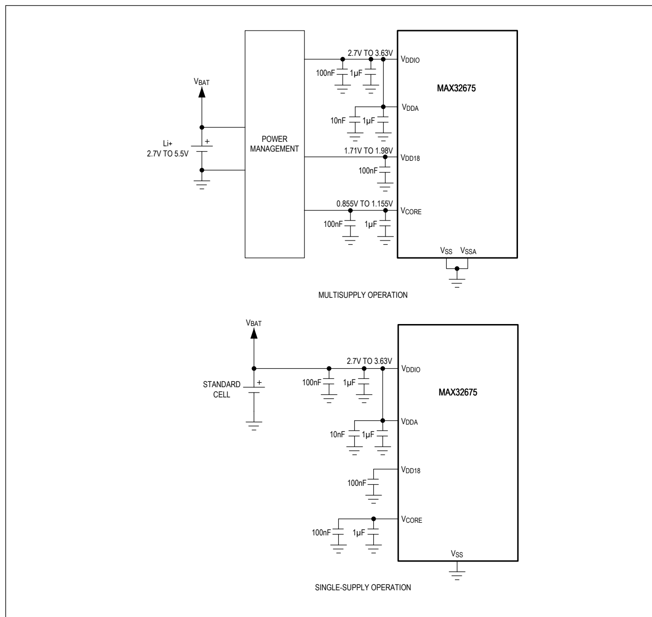
Figure 5. Power Supply Operation Modes
