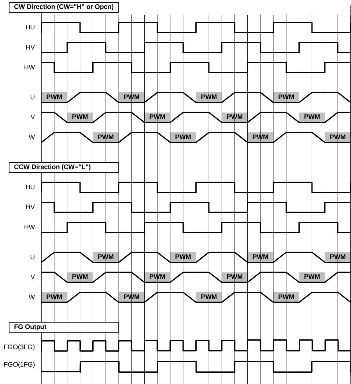
Figure 4. Timing Chart
