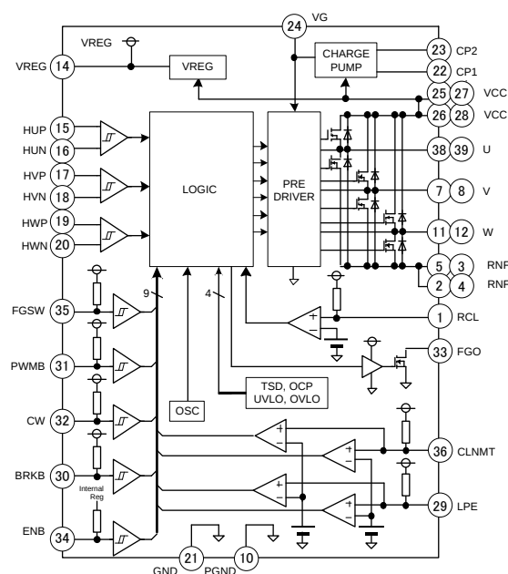
Figure 3. Block Diagram
