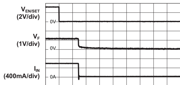
Turn-Off from 2x Mode Flash
