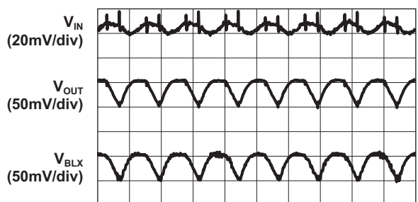
Backlight Operating Characteristics
