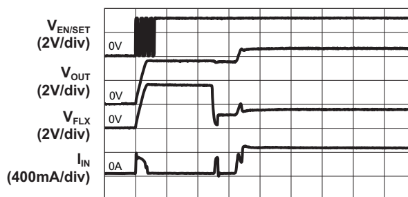
Turn-On to 1.5x Mode Flash
