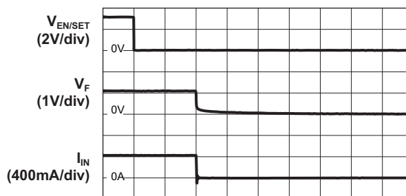
Turn-Off from 1.5x Mode Flash
