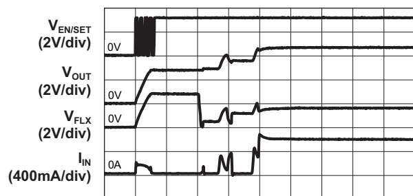
Turn-On to 2x Mode Flash
