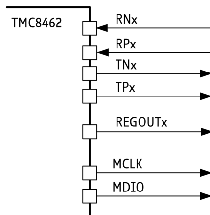
Figure 17: Physical bus interface pins
