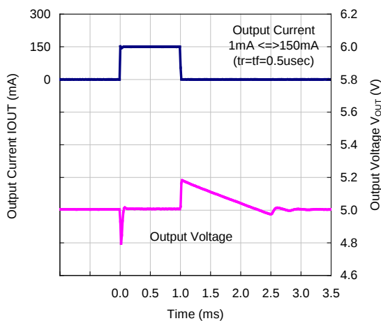
VR=5.0V, C_{OUT}=10\mu\text{F}
