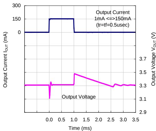
VR=3.3V, C_{OUT}=10\mu\text{F}
