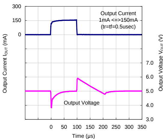
VR=5.0V, C_{OUT}=0.1\mu\text{F}
