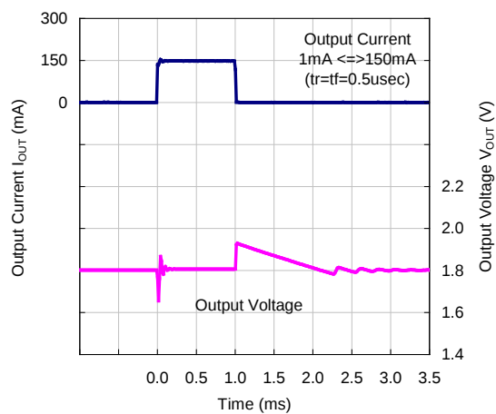
VR=1.8V, C_{OUT}=10\mu\text{F}
