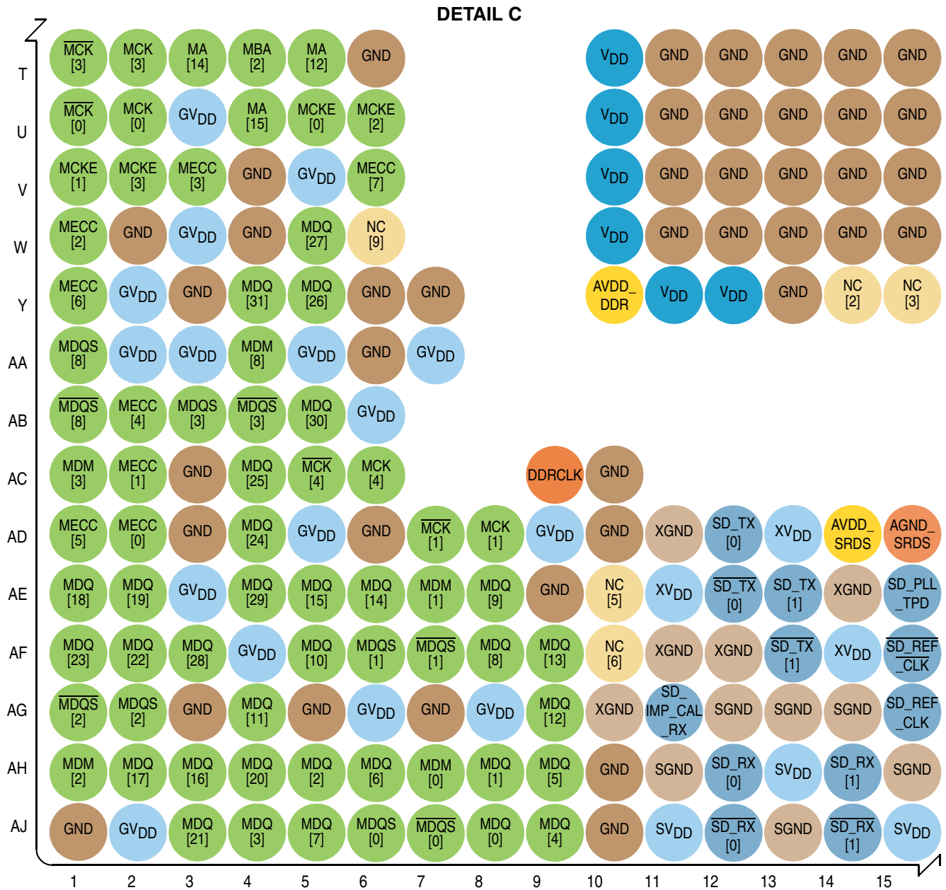
Figure 5. P2020 Ball Map—Detail C
