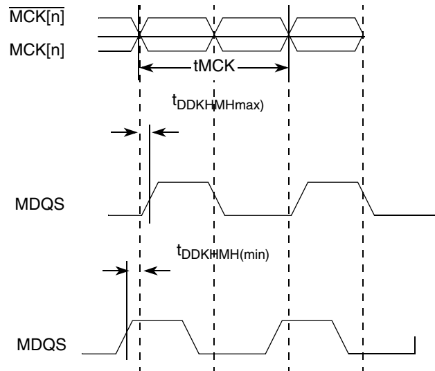
Figure 9. Timing Diagram for t_{\text{DDKMH}}
