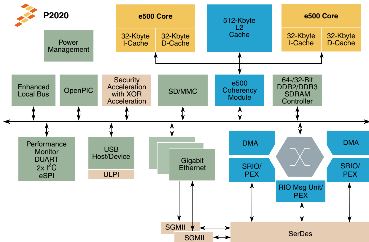
Figure 1. P2020 Block Diagram
