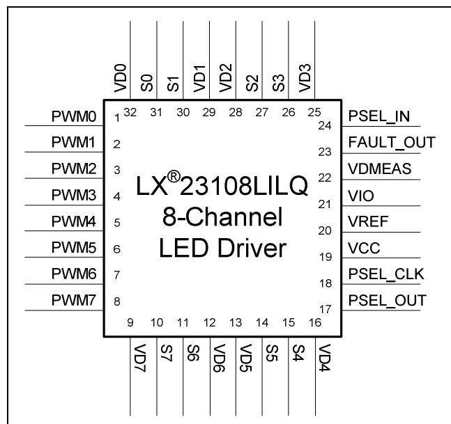
Figure 1: LX23108LILQ Pin Configuration
