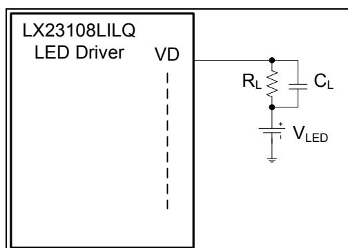
Figure 2: Test Circuit for Channel Rise/Fall Time Measurements
