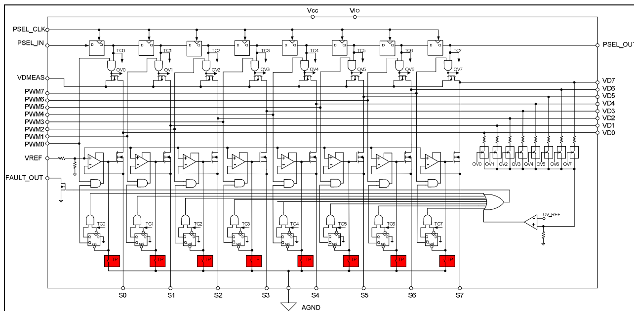
Figure 3: LX23108LILQ Block Diagram
