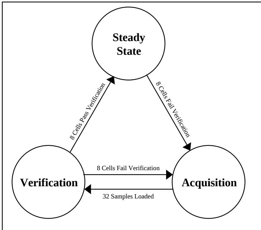
Figure 8-3 Receive DSS Scrambler Synchronization State Diagram
