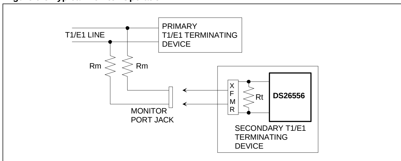
Figure 9-3 Typical Monitor Operation
