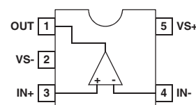
EL5193 (5 LD SOT-23) TOP VIEW
