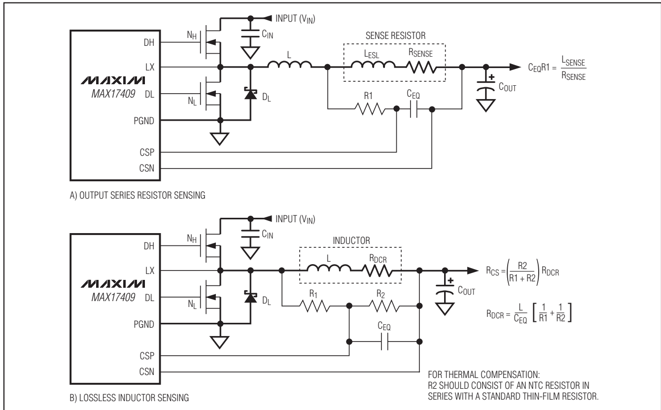
Figure 3. Current-Sense Methods
