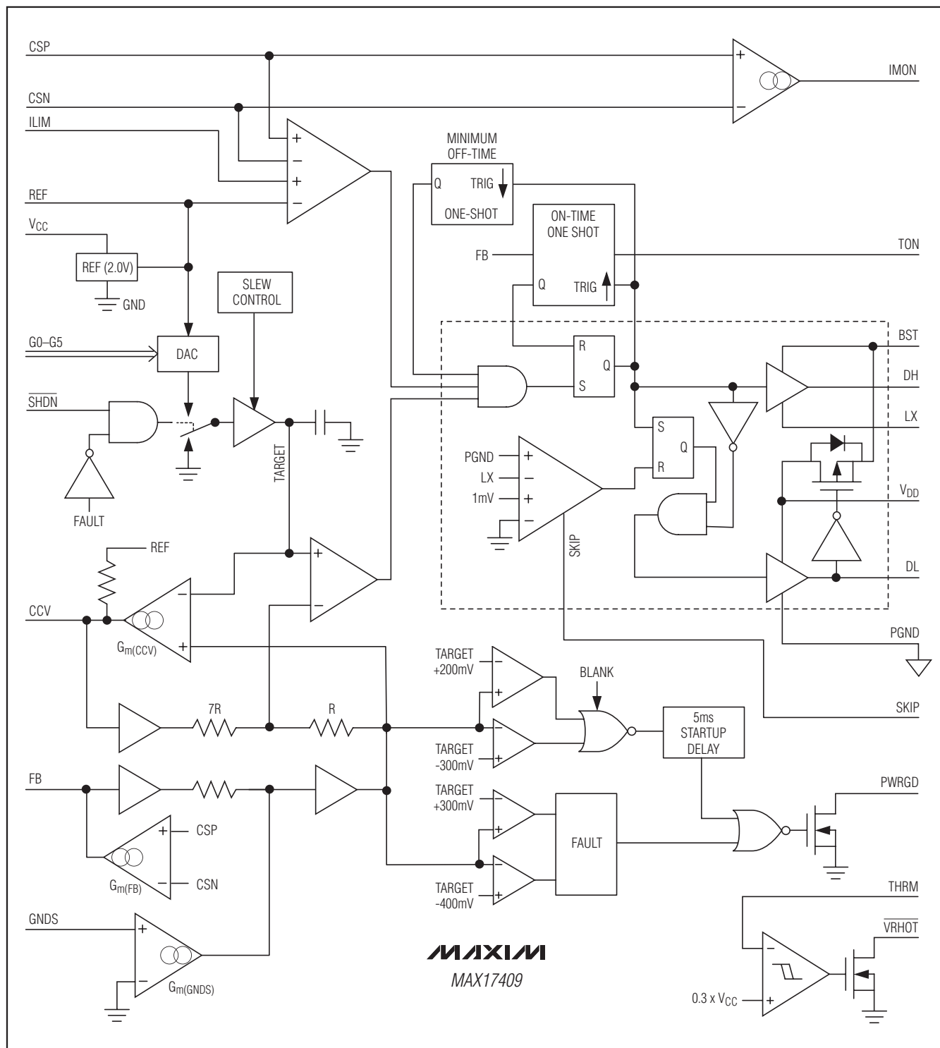
Figure 2. Functional Diagram
