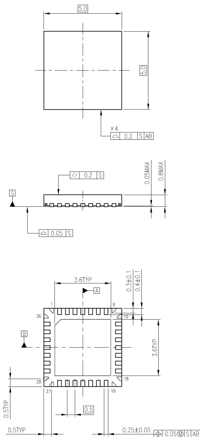
Figure 13.1 Package Dimensions
