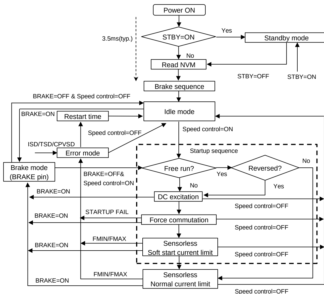
Figure 8.1 Flowchart of basic operation
