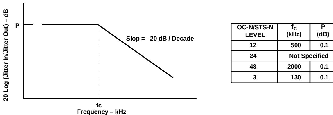
Figure 2. Jitter Transfer
