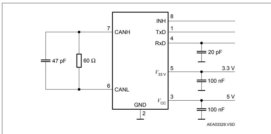
Figure 8 Test Circuit for Dynamic Characteristics (GV33 Version)
