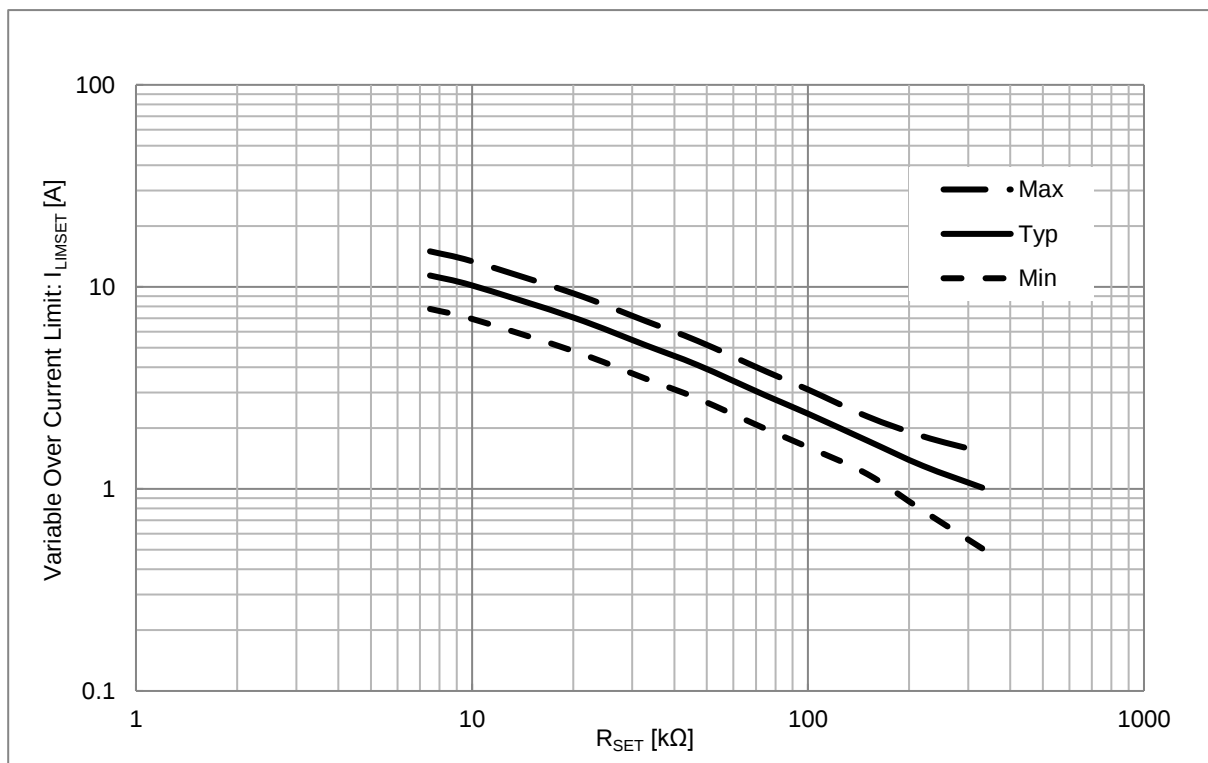
Figure 36. Variable Over Current Limit vs R_{\text{SET}}
