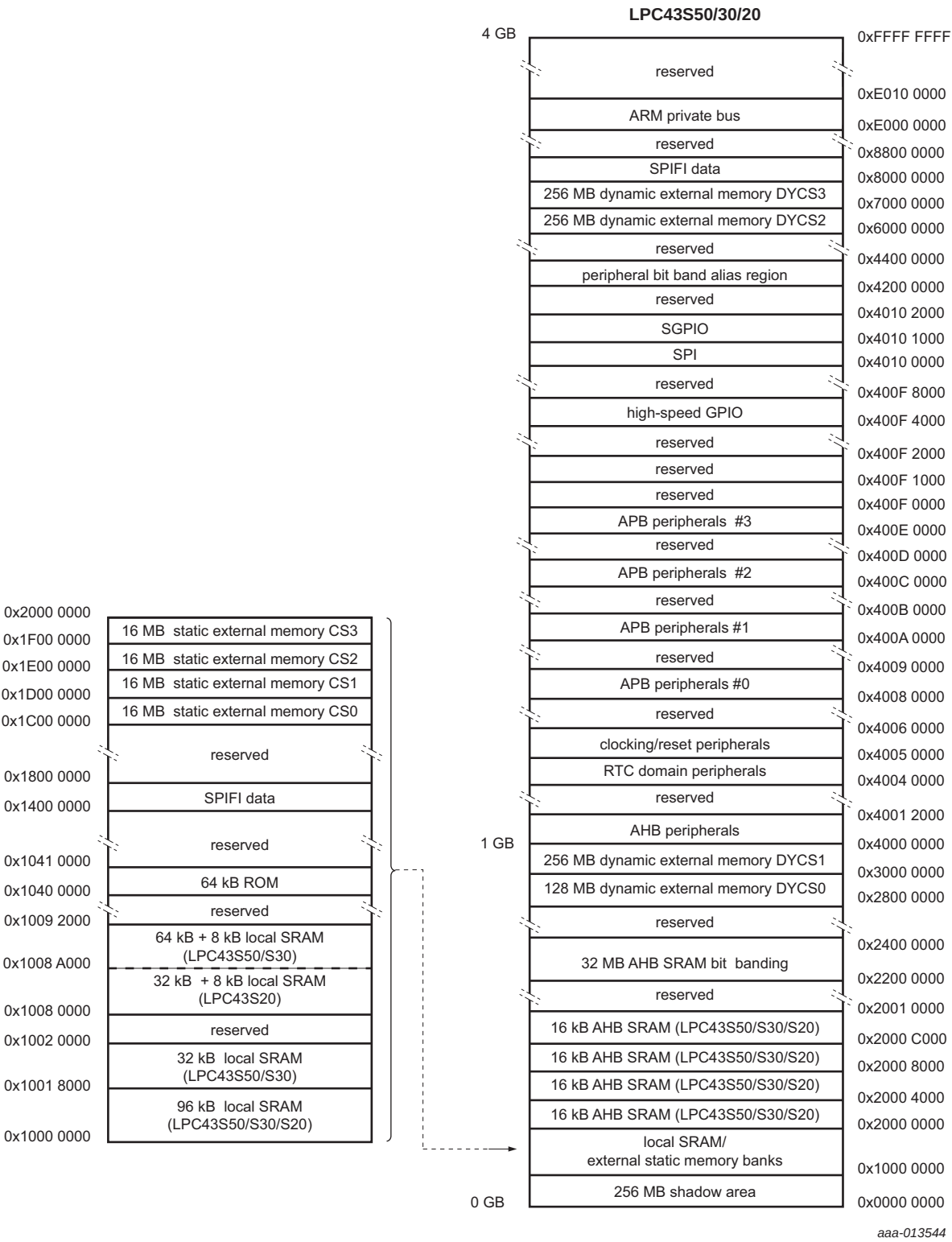
Fig 7. LPC43S50/S30/S20 Memory mapping (overview)
