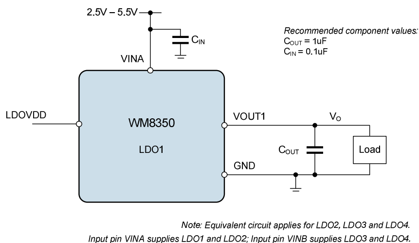
Figure 71 LDO Regulator Connections
