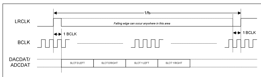
Figure 60 DSP/PCM Mode A, Slave Mode with TDM
