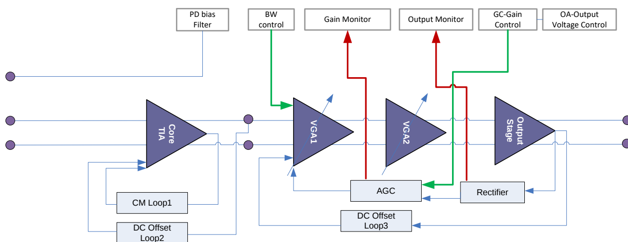
Figure 1. Block Diagram
