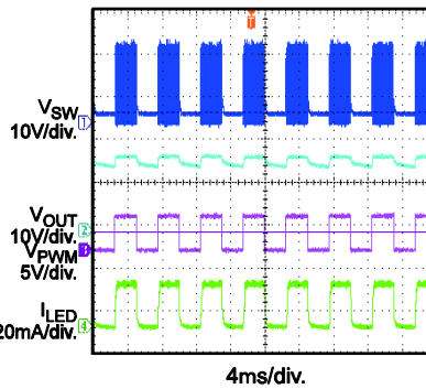
PWM Dimming
