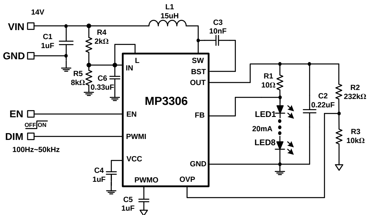
Figure 8— The application when V_{in} > 12V
