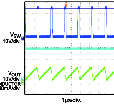
Steady State
