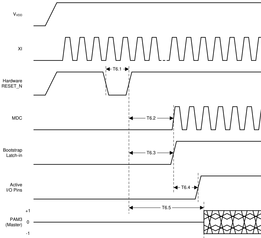
Figure 7-2. Reset Timing
