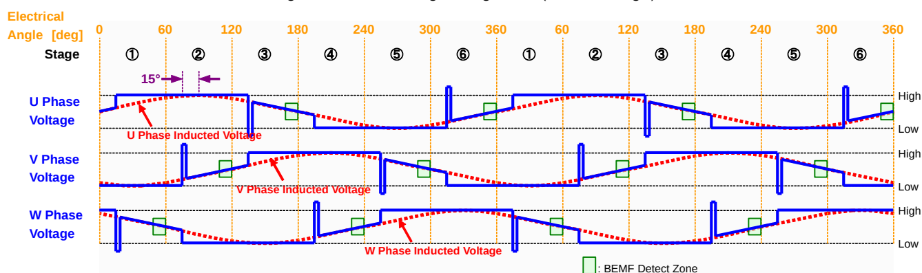
Figure 43. 15° Setting Timing Chart (LASEL = Middle)
