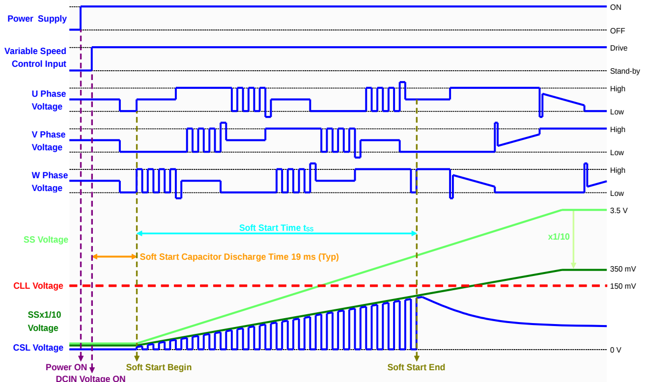
Figure 50. Soft Start PMM Operation Timing Chart when Power ON (variable speed control input)
