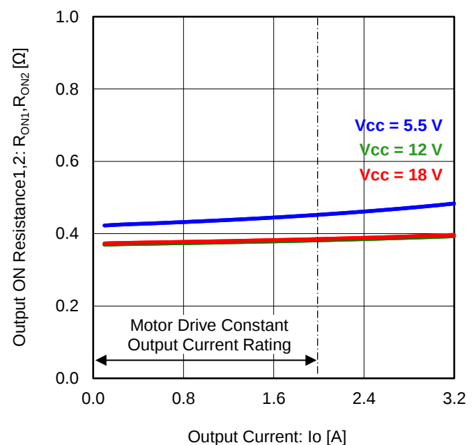
Figure 4. Motor Drive Output ON Resistance1,2 (High / Low Total) vs Motor Drive Output Current T_j = 25 \text{ °C} (Supply Voltage Comparison)
