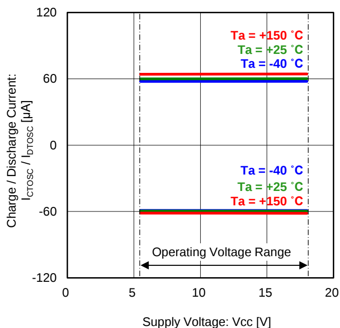
Figure 14. TOSC Charge / Discharge Current vs Supply Voltage
