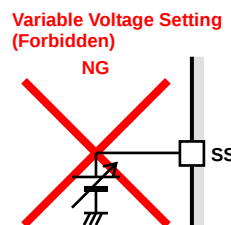
Figure 53. Variable Voltage Input to the SS pin is forbidden
