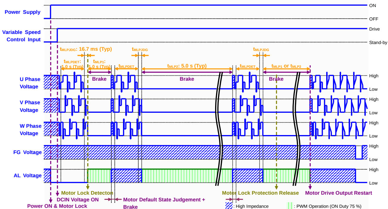
Figure 62. Motor Lock Protection Timing Chart (During the start-up mode)
