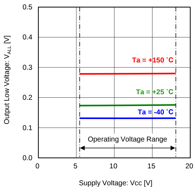
Figure 10. AL Output Low Voltage vs Supply Voltage
