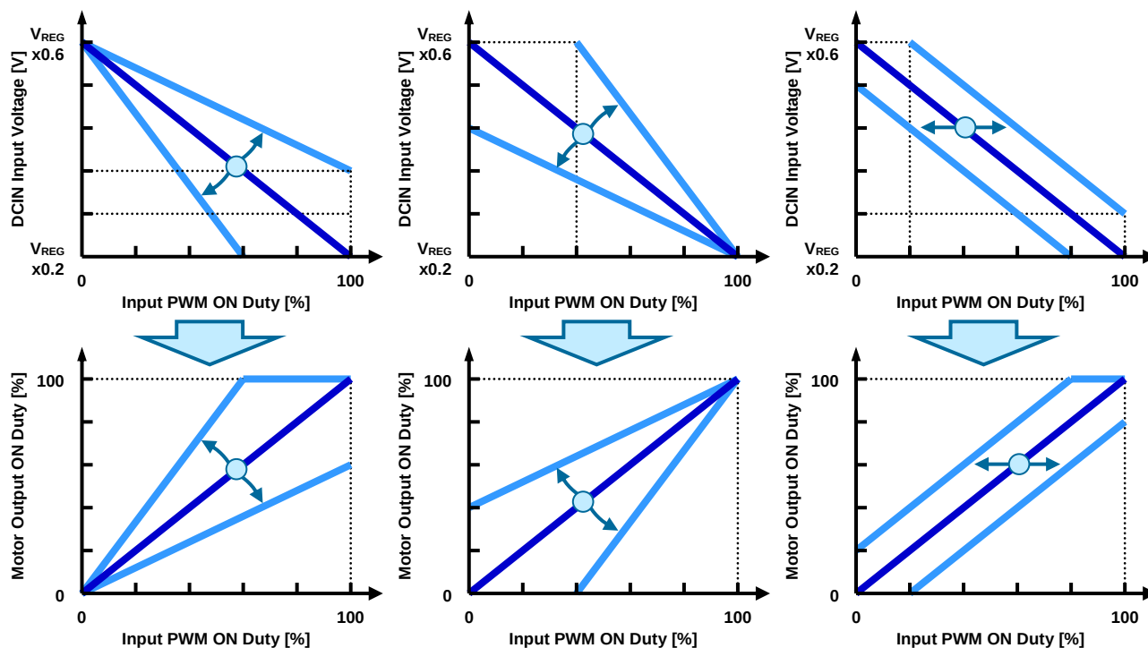
Figure 35. Example of Variable Speed Control Slope and Shift Setting
