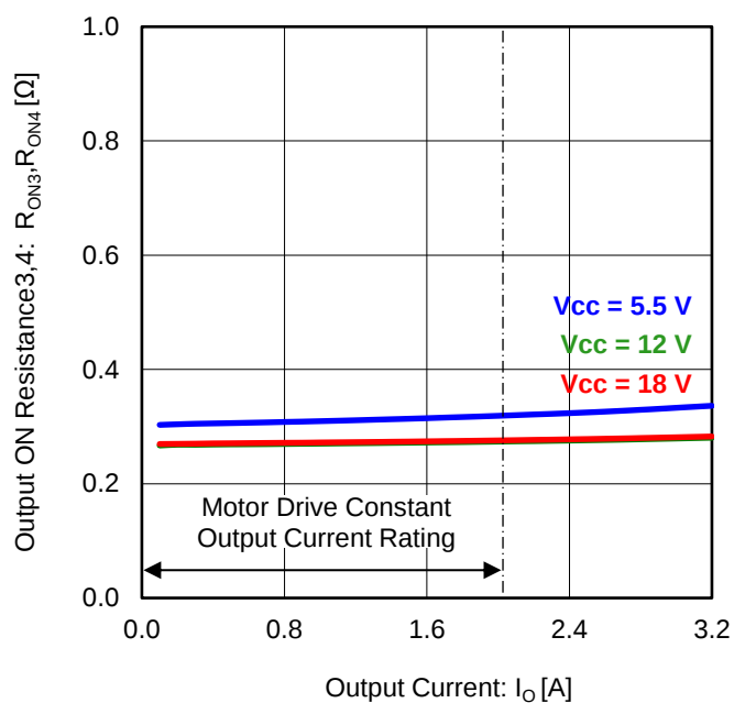
Figure 5. Motor Drive Output ON Resistance3,4 (High / Low Total) vs Motor Drive Output Current T_j = -40\text{ }^{\circ}\text{C} (Supply Voltage Comparison)
