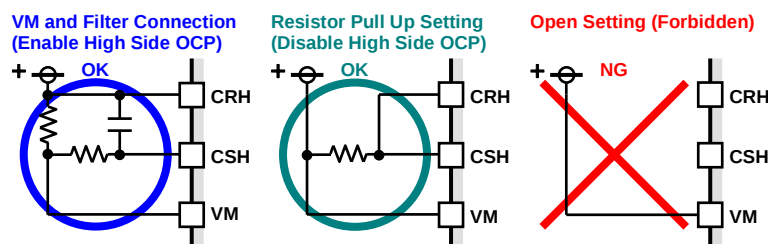
Figure 66. High Side Over Current Protection Function
