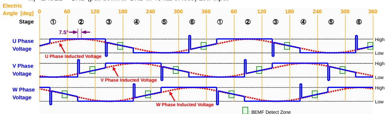
Figure 42. 7.5° Setting Timing Chart (LASEL = High)
