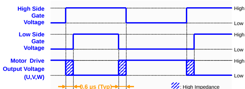
Figure 40. Synchronous Rectification Timing Chart when PWM Operation
