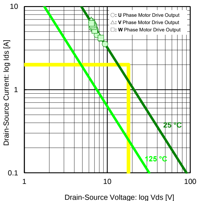
Figure 89. Drain-Source Current vs Drain-Source Voltage Motor Drive Output Low Side DMOS ASO P_w = 100\text{ ms} (Temperature Derating)
