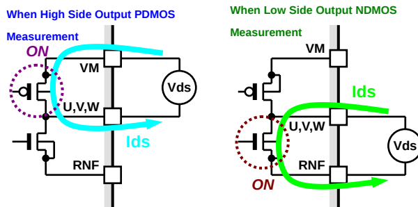
Figure 77. ASO Measure Schematic Diagram
