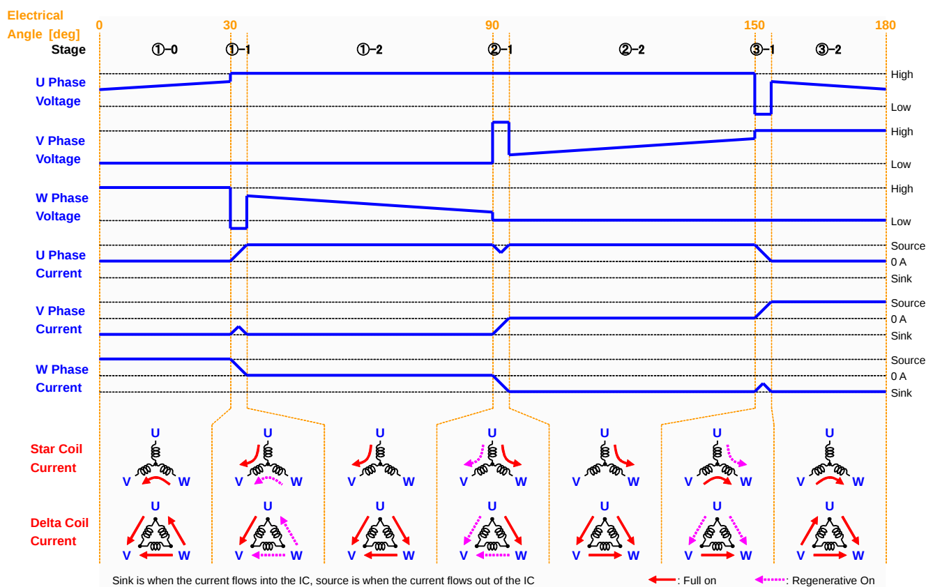
Figure 31. Motor Coil Current Change when 120° Commutation Drive
