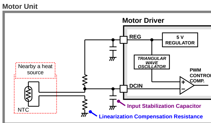
Figure 36. Temperature Control Application
