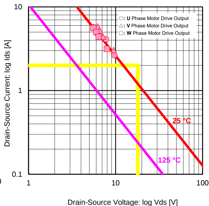
Figure 83. Drain-Source Current vs Drain-Source Voltage Motor Drive Output High Side DMOS ASO Pw = 500 ms (Temperature Derating)
