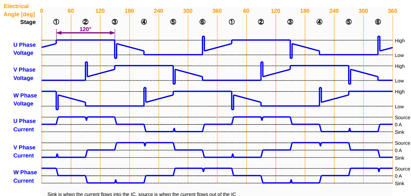
Figure 30. 120° Commutation Drive Timing Chart
