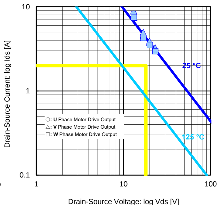
Figure 85. Drain-Source Current vs Drain-Source Voltage Motor Drive Output High Side DMOS ASO Pw = 10 ms (Temperature Derating)
