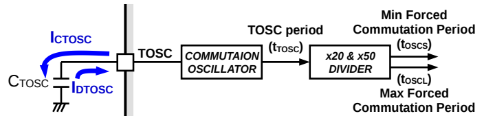
Figure 26. TOSC Capacitor and IC Internal Circuit Diagram
