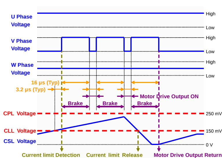
Figure 47. Current Limit PWM Operation Timing Chart 2
