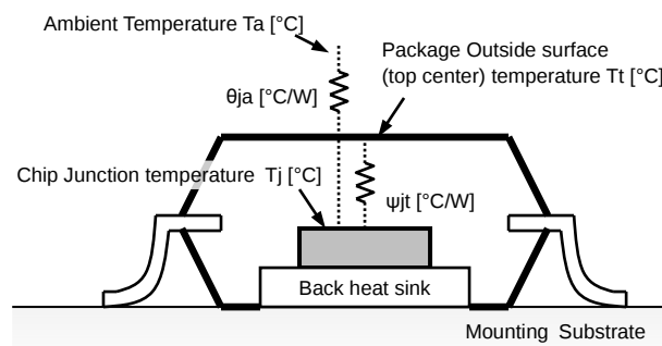
Figure 73. Thermal Resistance Model of package
