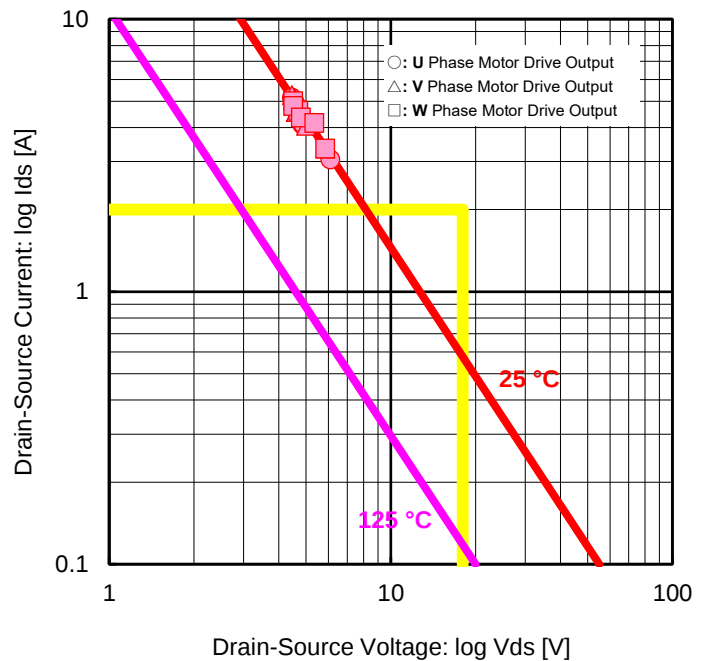
Figure 88. Drain-Source Current vs Drain-Source Voltage Motor Drive Output Low Side DMOS ASO P_w = 500\text{ ms} (Temperature Derating)
