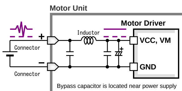
Figure 98. Power Supply Stabilization Measure (LC Filter)
