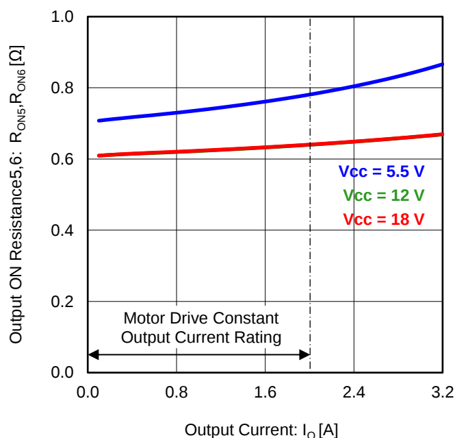
Figure 6. Motor Drive Output ON Resistance5,6 (High / Low Total) vs Motor Drive Output Current T_j = 150\text{ }^{\circ}\text{C} (Supply Voltage Comparison)
