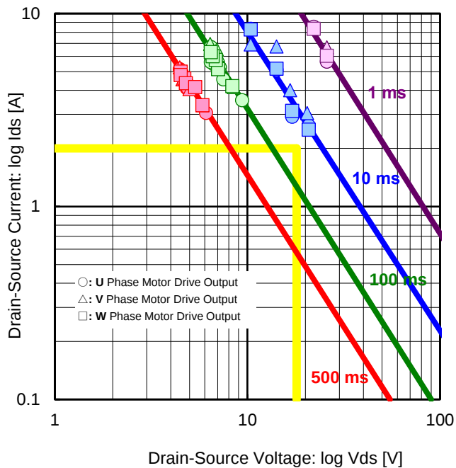
Figure 87. Drain-Source Current vs Drain-Source Voltage Motor Drive Output Low Side DMOS ASO T_a = 25\text{ }^{\circ}\text{C} (Input Time Comparison)
