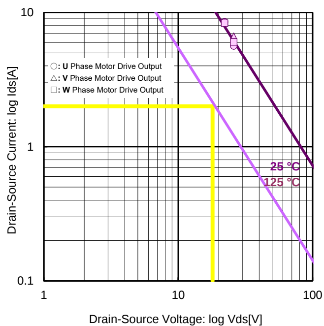
Figure 91. Drain-Source Current vs Drain-Source Voltage Motor Drive Output Low Side DMOS ASO P_w = 1 \text{ ms} (Temperature Derating)
