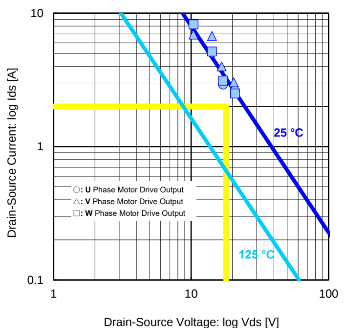
Figure 90. Drain-Source Current vs Drain-Source Voltage Motor Drive Output Low Side DMOS ASO P_w = 10\text{ ms} (Temperature Derating)
