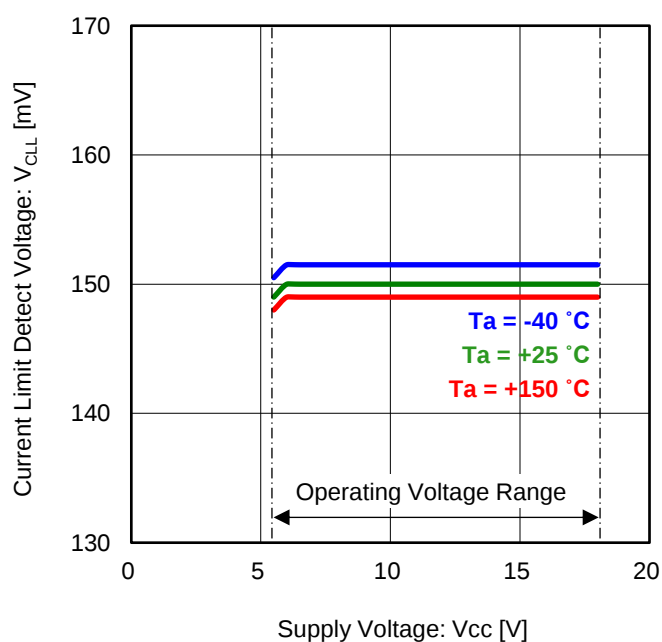
Figure 16. Current Limit Detect Voltage vs Supply Voltage
