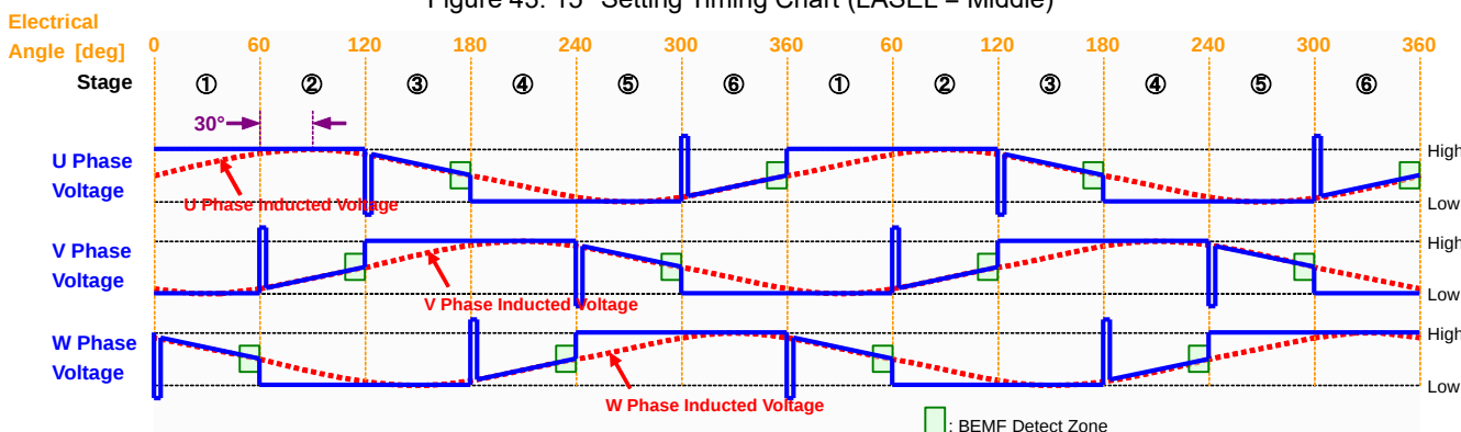
Figure 44. 30° Setting Timing Chart (LASEL = Low)
