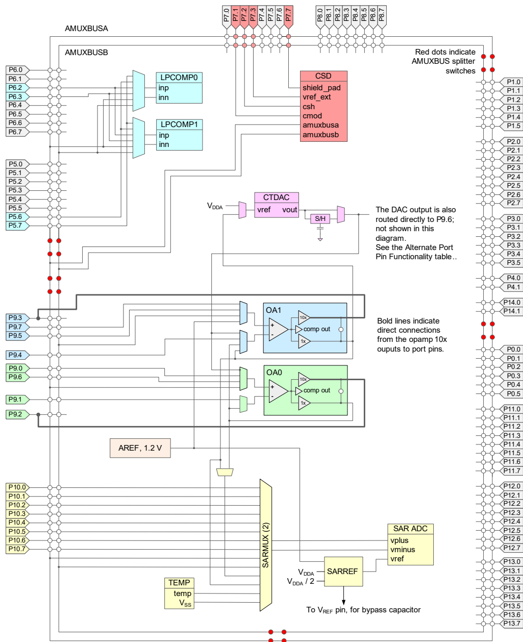
Figure 6. Analog Subsystem
