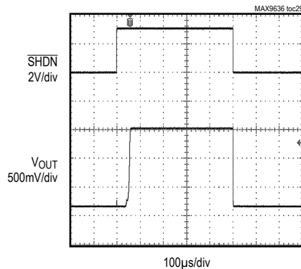
TURN-ON TIME
