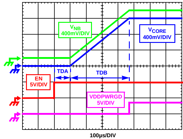
FIGURE 11. SOFT-START WAVEFORMS
